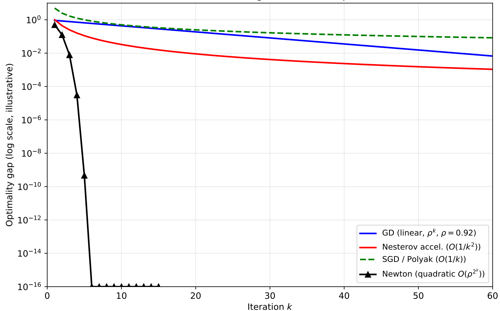
Theoretical Convergence Rate Comparison
