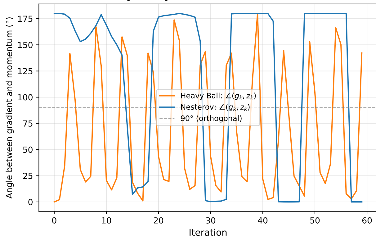
Alignment: gradient vs momentum direction
