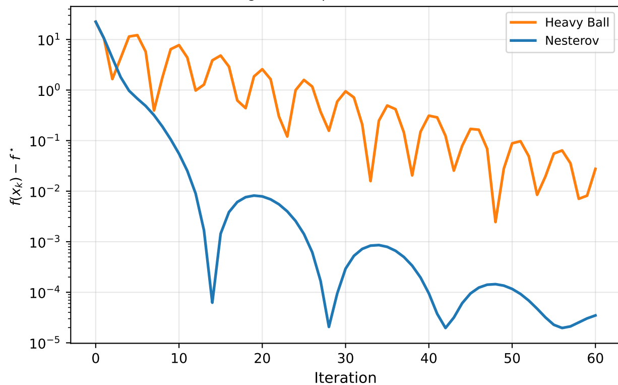
Convergence comparison (same \alpha = 0.035 )
