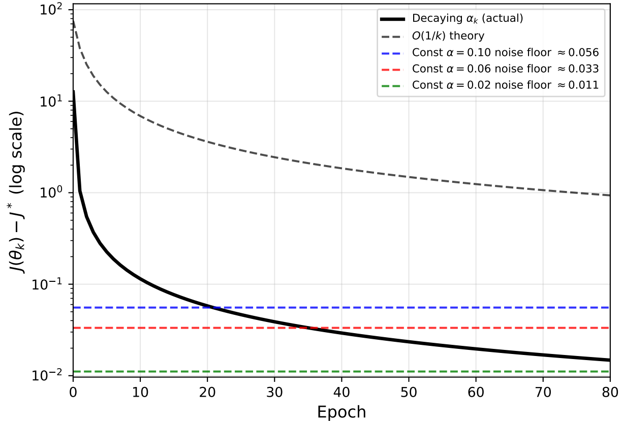
Q2: SGD Noise Floor vs Decaying Step Horizontal lines = constant- \alpha asymptotic limits
