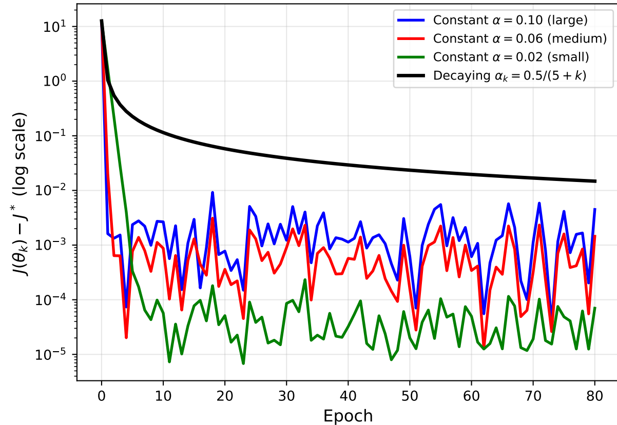
Q2: SGD Convergence — Constant vs Decaying Step Size Benchmark A, batch size b = 20 , 80 epochs
