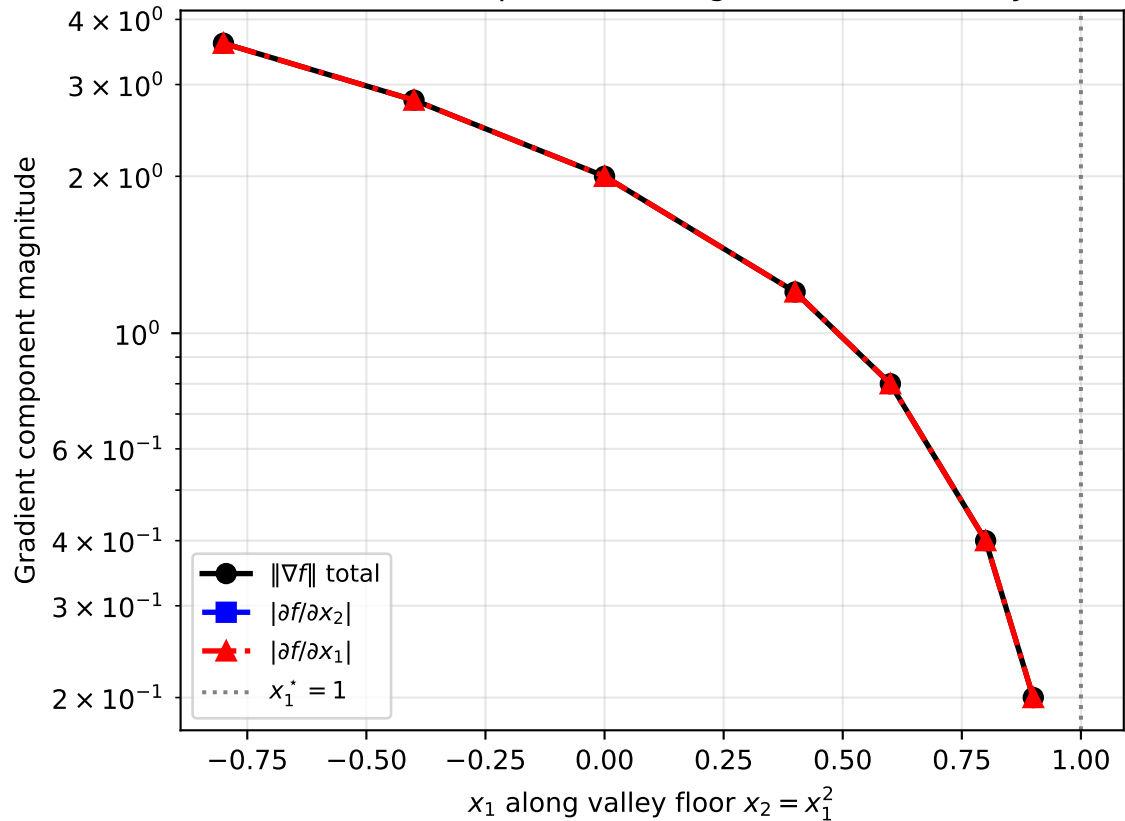
Gradient Components Along Rosenbrock Valley
