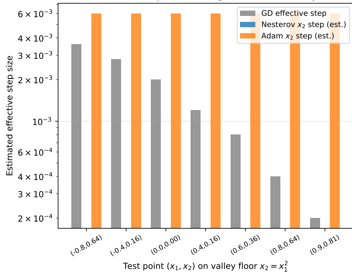
Effective Step Sizes Along Rosenbrock Valley
