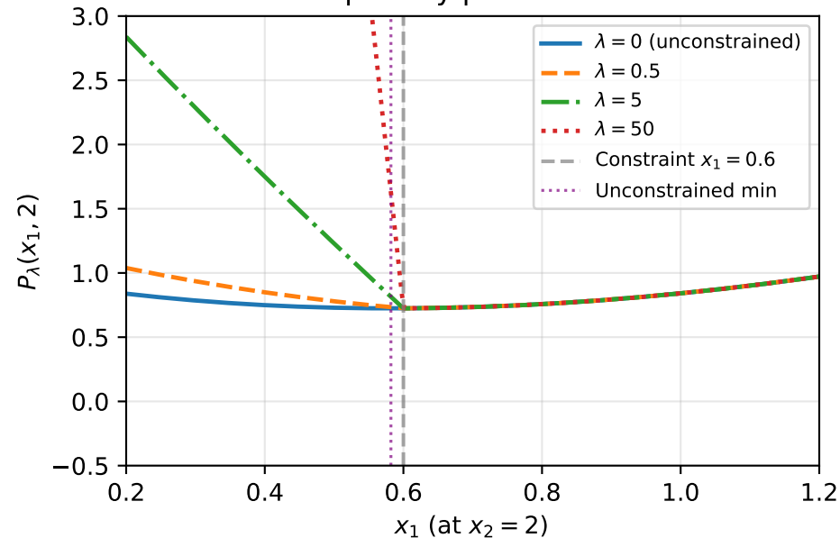
Penalty function landscape vs penalty parameter \lambda
