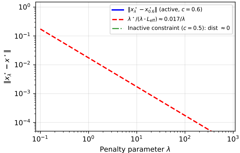
O(1/\lambda) convergence for active constraint (inactive: exact feasibility for any \lambda )
