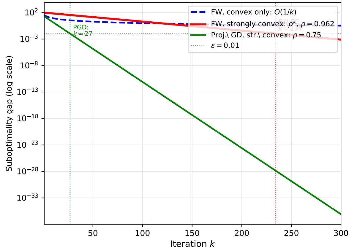
FW Linear Convergence under Strong Convexity (\mu = 0.5, L = 2.0, D = 5.0; \text{PGD: } \rho = 0.75, \text{FW-SC: } \rho = 0.962)
