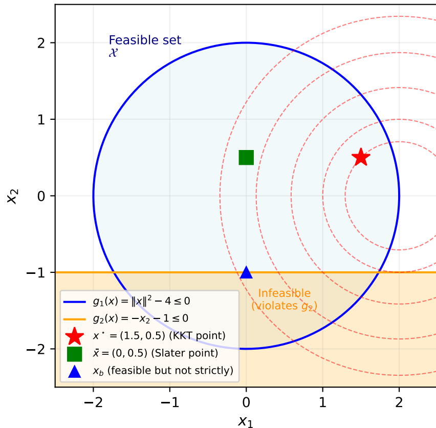
Slater's Condition for Strong Duality (Slater point \bar{x} in interior of \mathcal{X} \rightarrow strong duality)
