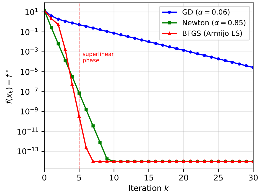
(a) Convergence on Benchmark B
