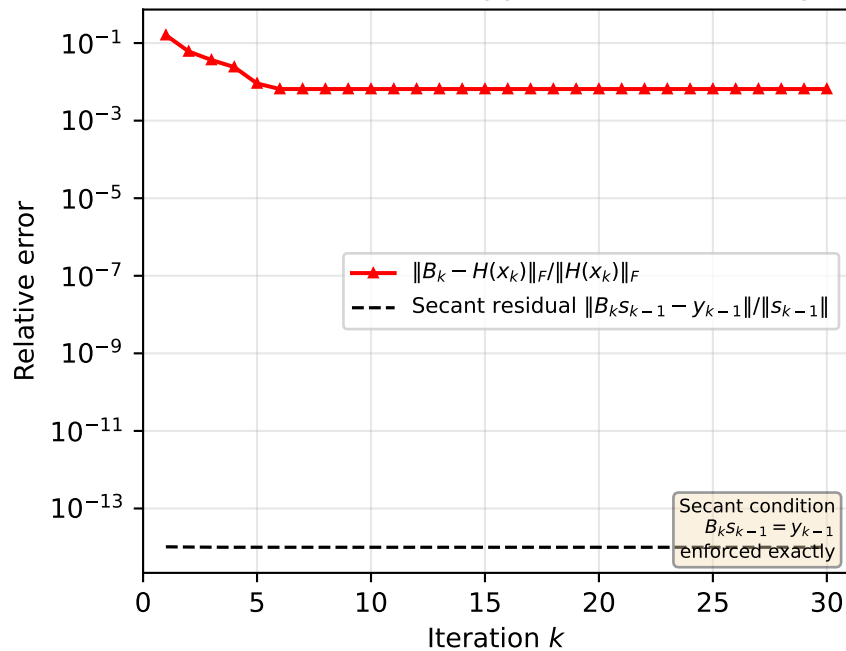
(b) BFGS Hessian Approximation Quality
