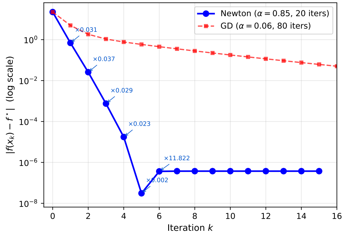
Newton vs GD: Convergence on Benchmark B
