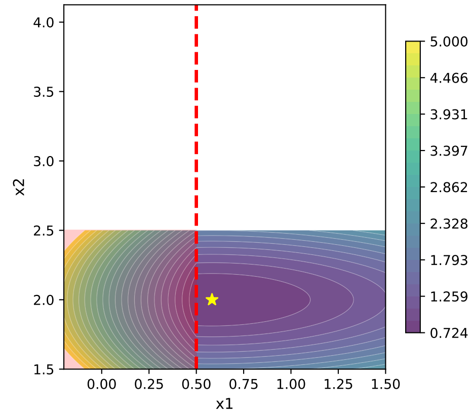
Q5: Penalised Objective (lambda=4.5 (strong penalty))
