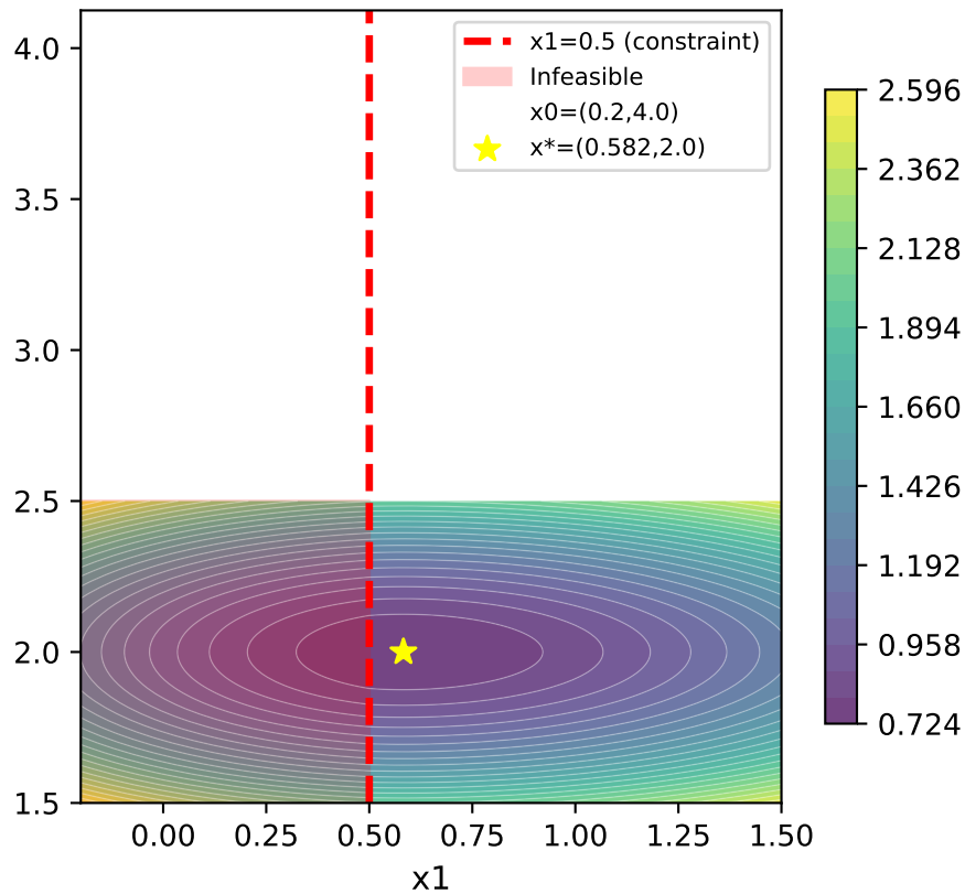
Q5: Penalised Objective (lambda=0.15 (weak penalty))
