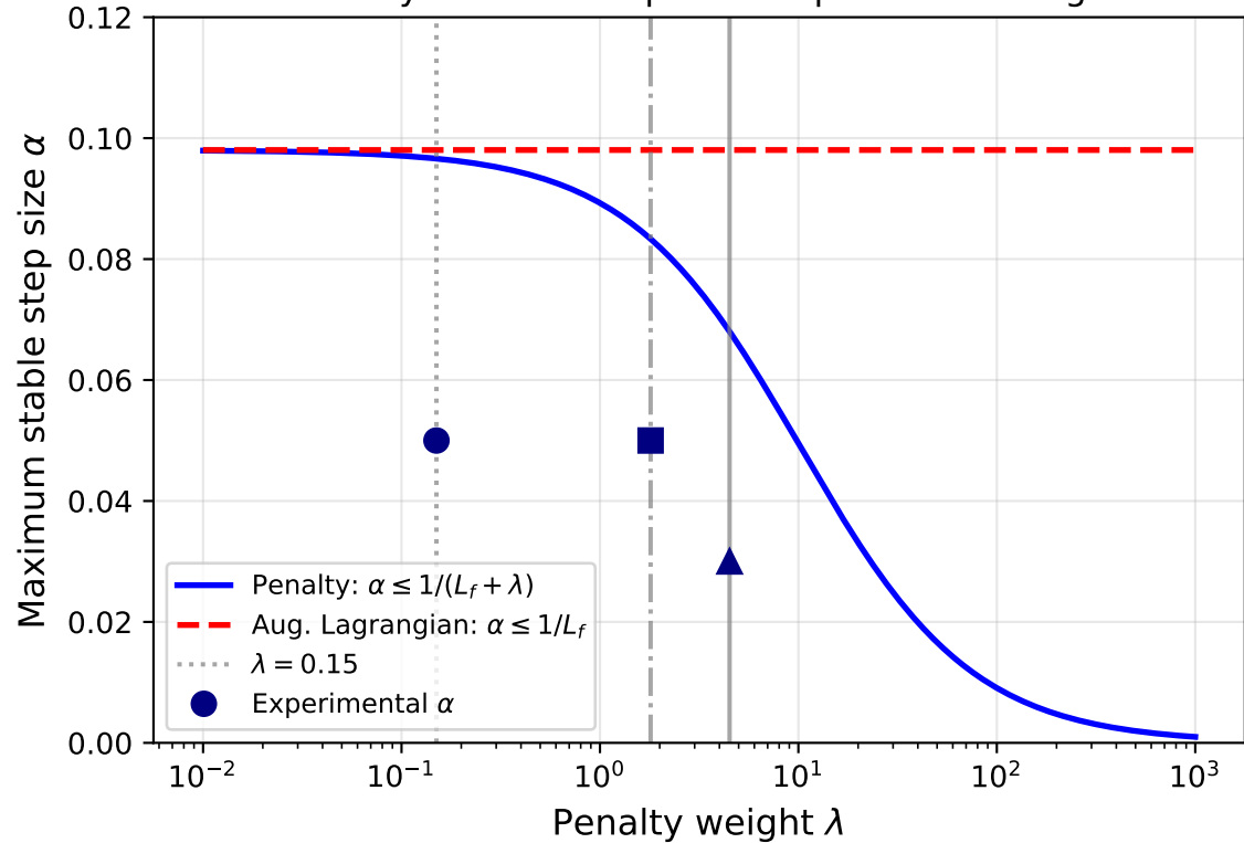
Penalty Method: Required Step Size Shrinkage
