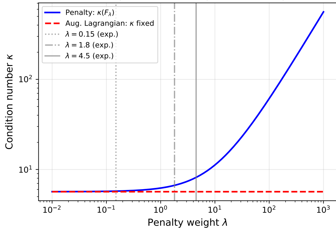
Penalty Method: Growing Ill-Conditioning
