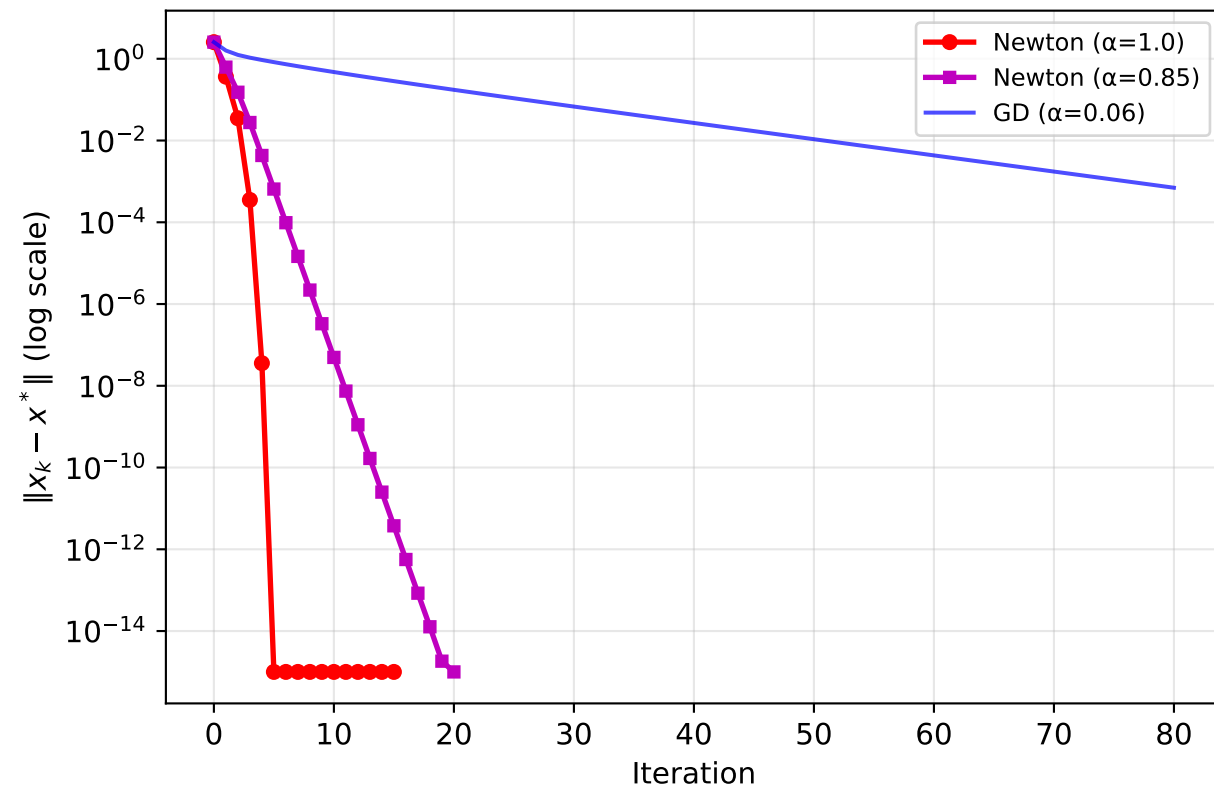
Newton vs GD — Benchmark B ( \kappa \approx 6.9 )
