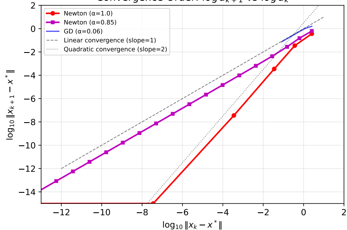
Convergence Order: \log d_{k+1} vs \log d_k
