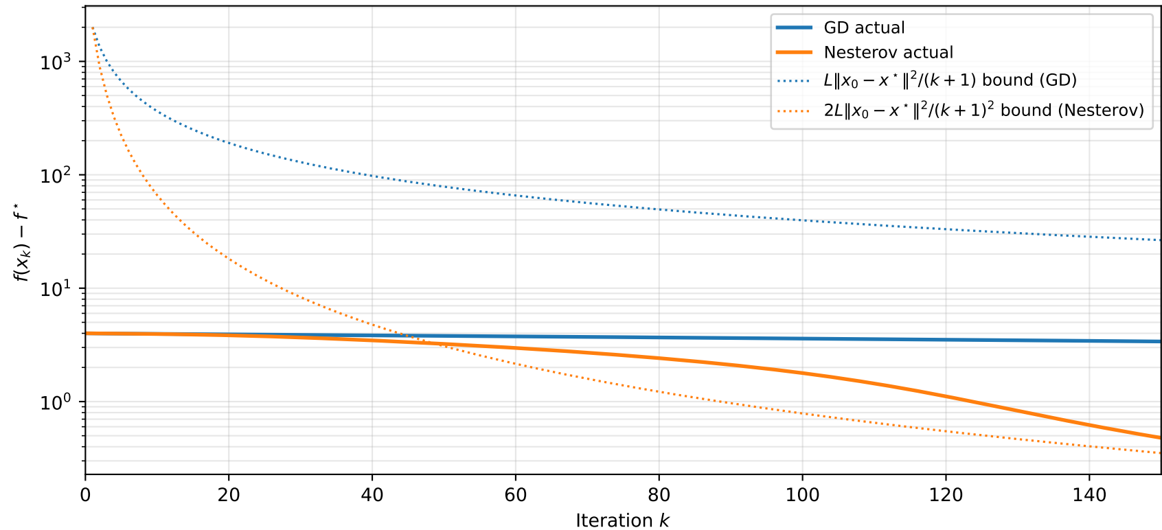
GD vs Nesterov on Benchmark C (Rosenbrock): Actual vs Theoretical Bounds
