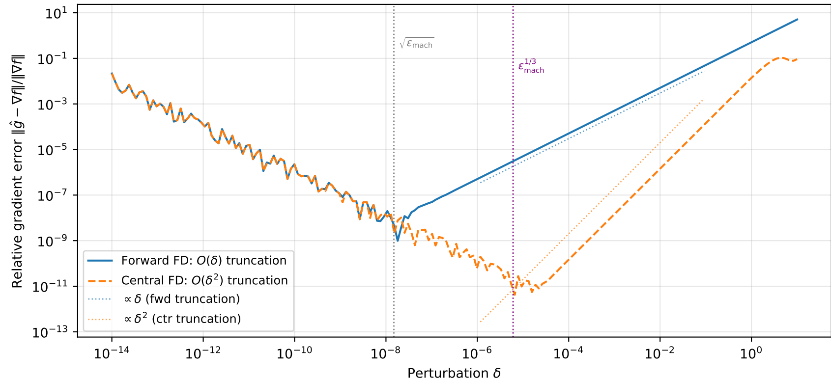
Forward vs Central Finite Differences on Benchmark B at x = (0.5, 3.0)
