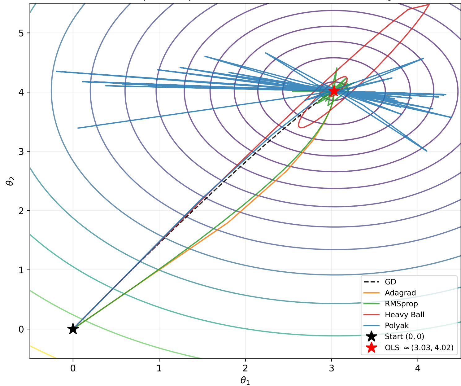
Q1: Parameter-Space Trajectories — Benchmark A (Linear Regression)
