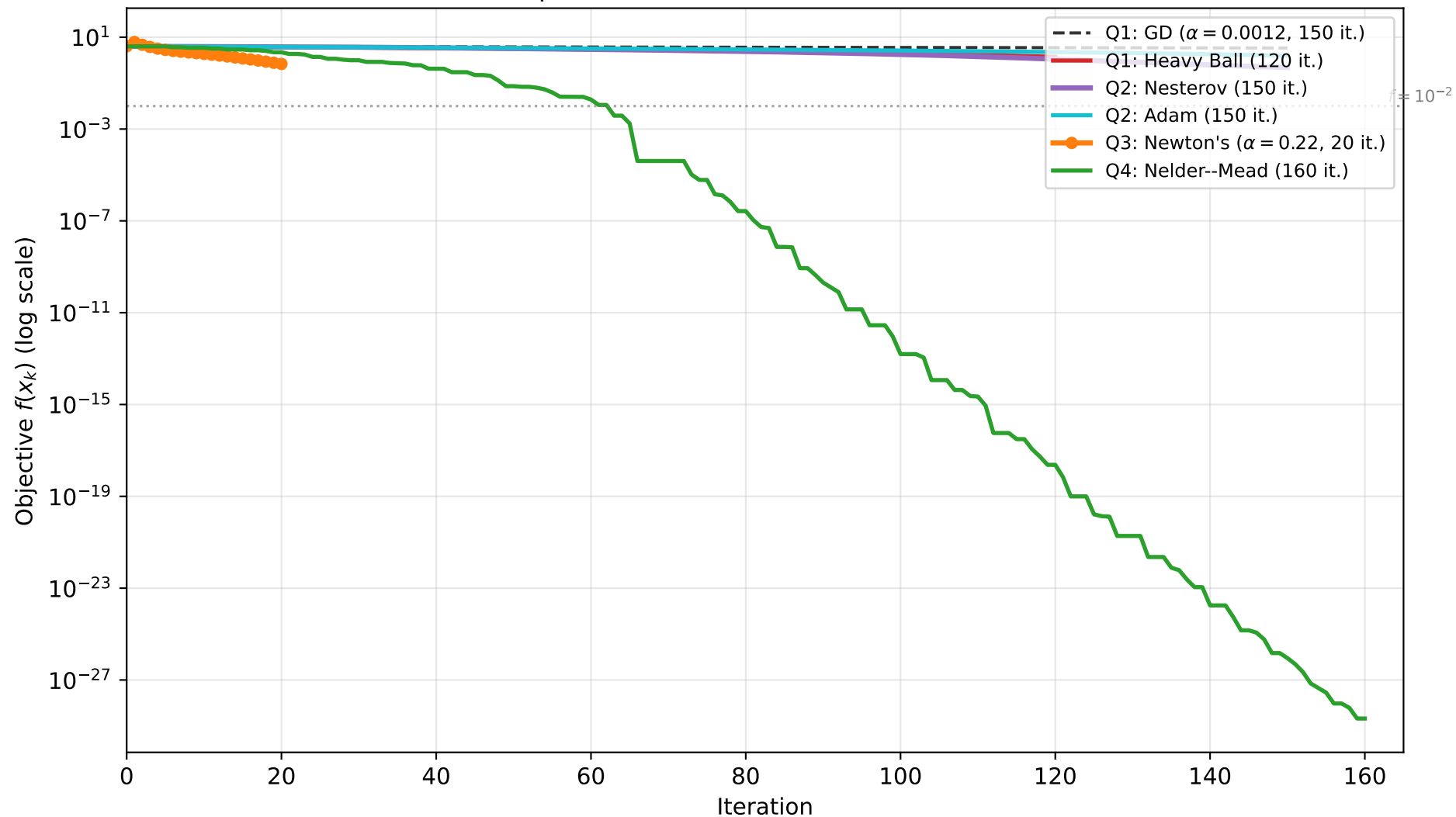
Cross-Question Comparison: Best Methods on Rosenbrock (Benchmark C)
