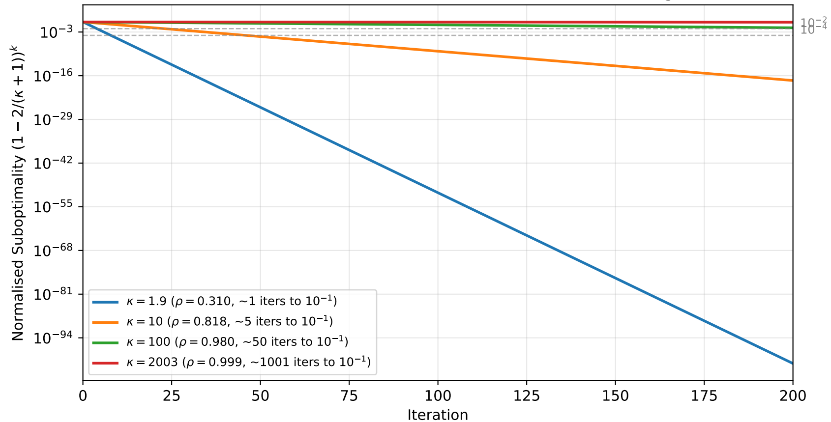
Effect of Condition Number \kappa on Gradient Descent Convergence
