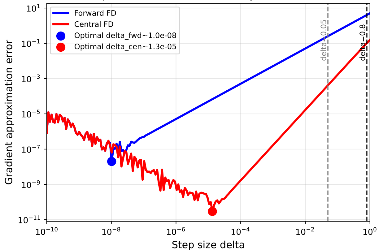
Optimal Delta and Error at Assignment Values
