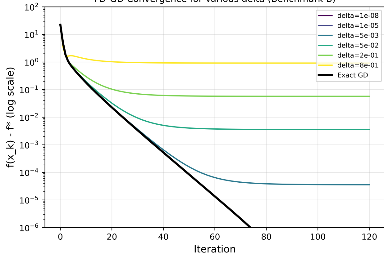
FD-GD Convergence for Various delta (Benchmark B)
