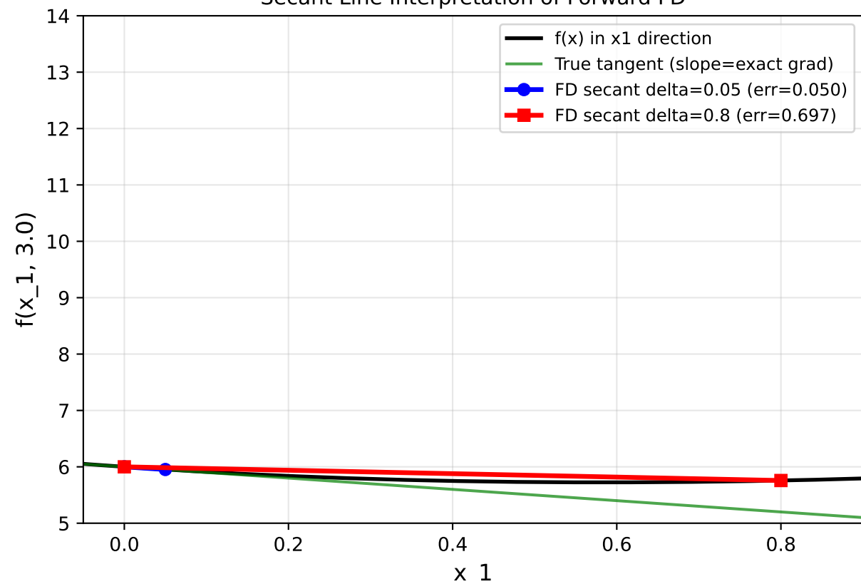
Secant Line Interpretation of Forward FD
