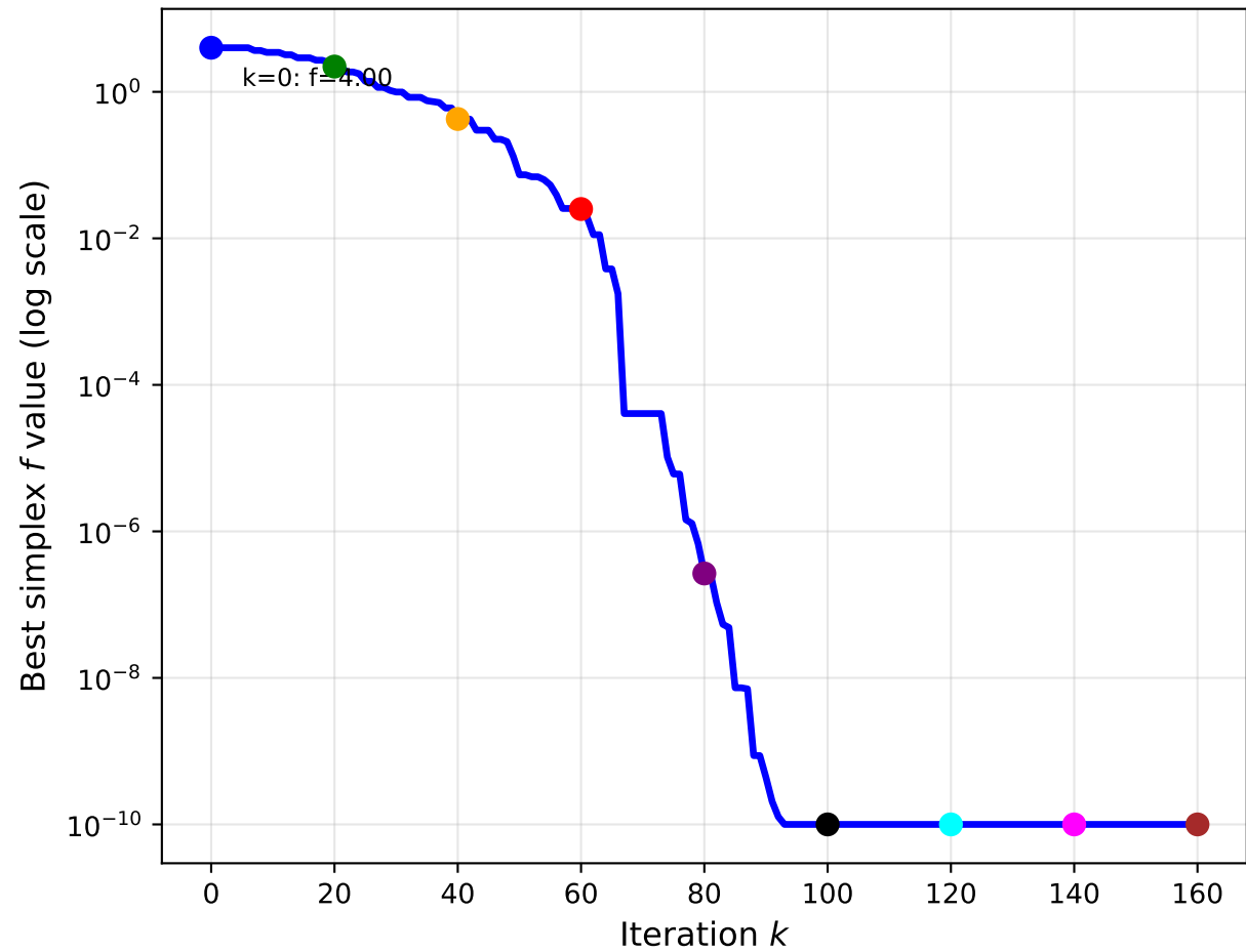
Nelder-Mead Convergence (Best vertex objective value)
