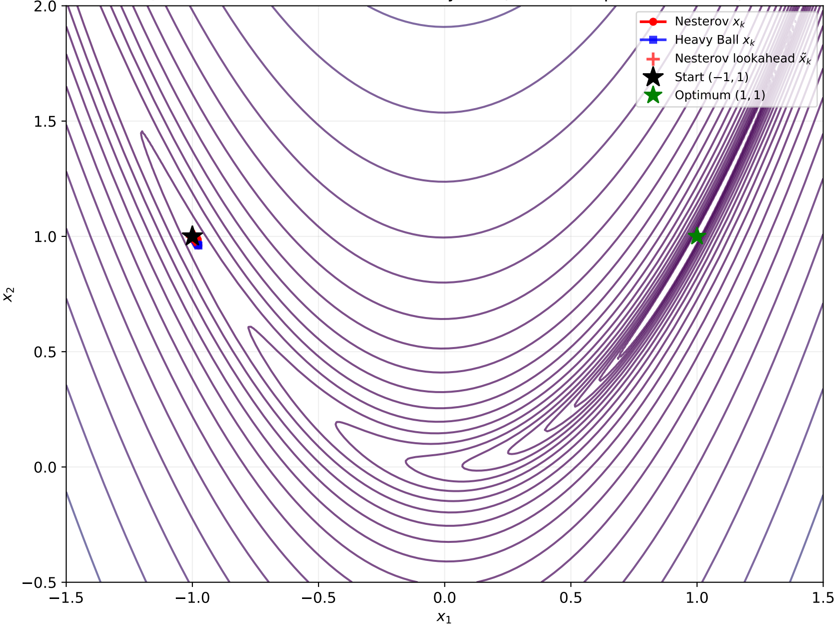
Q2: Nesterov Lookahead vs. Heavy Ball (first 14 steps, Rosenbrock)
