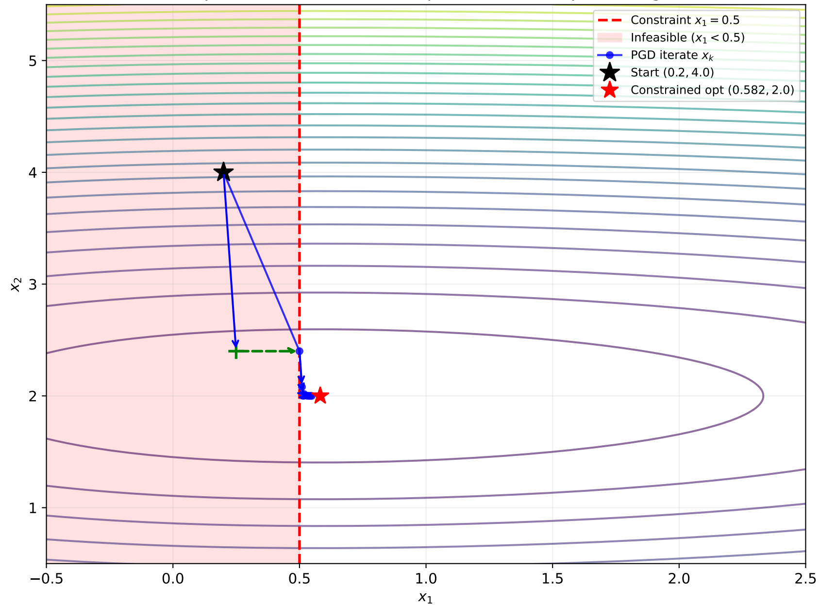
Q5: Projected GD — Gradient Steps (blue) and Projections (green)
