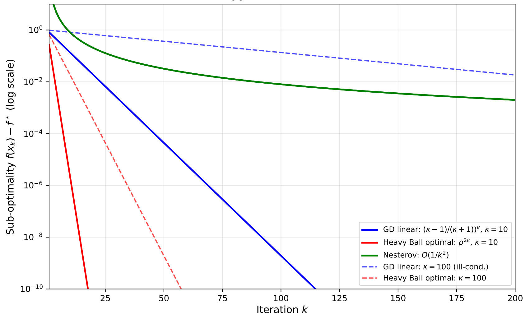
Theoretical Convergence Rates: GD vs Heavy Ball vs Nesterov (smooth strongly convex, \kappa = \text{condition number} )
