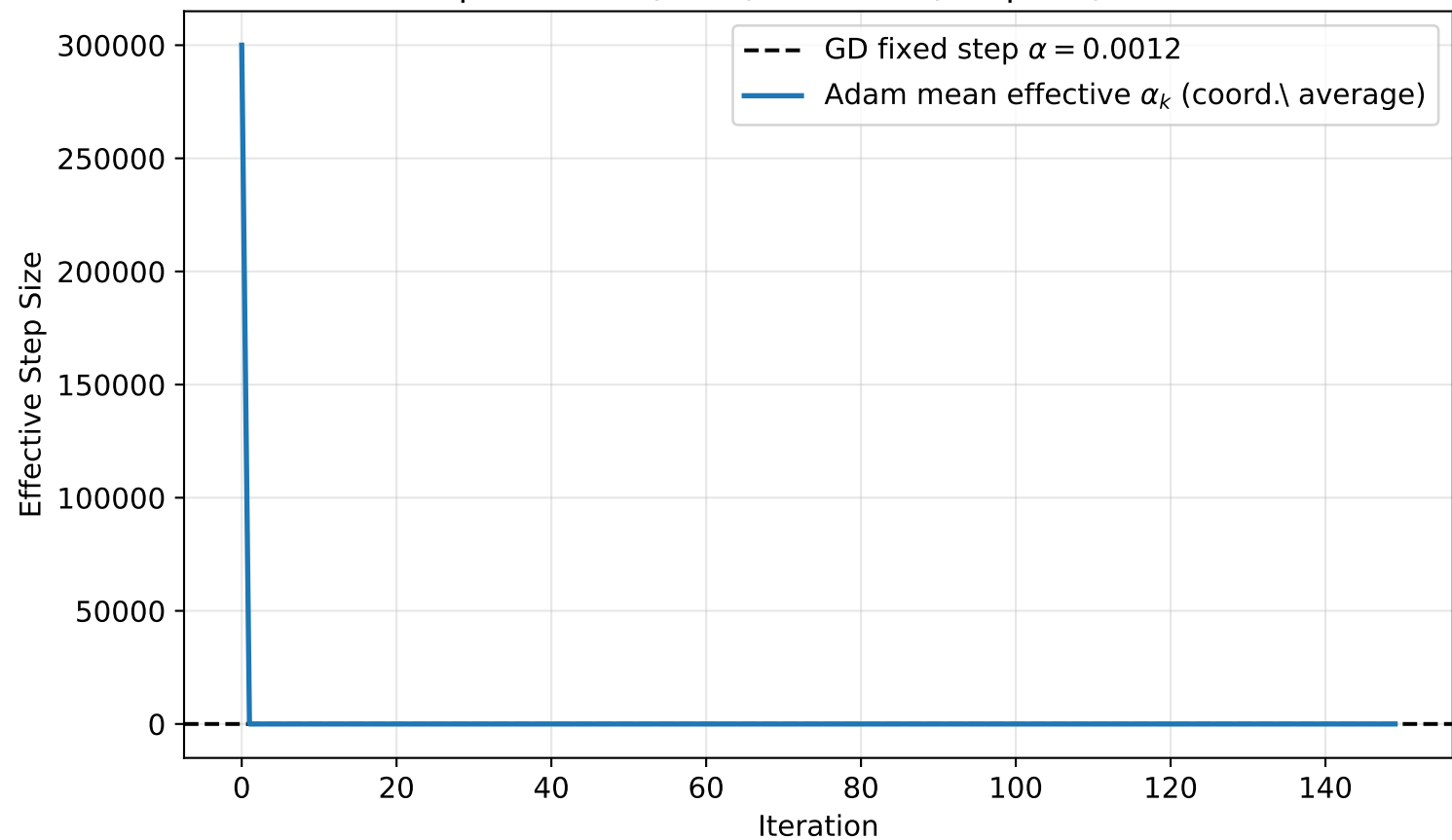
Effective Step Size: GD (fixed) vs Adam (adaptive) — Benchmark C
