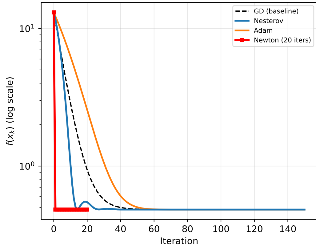
Benchmark A (Linear Regression)
