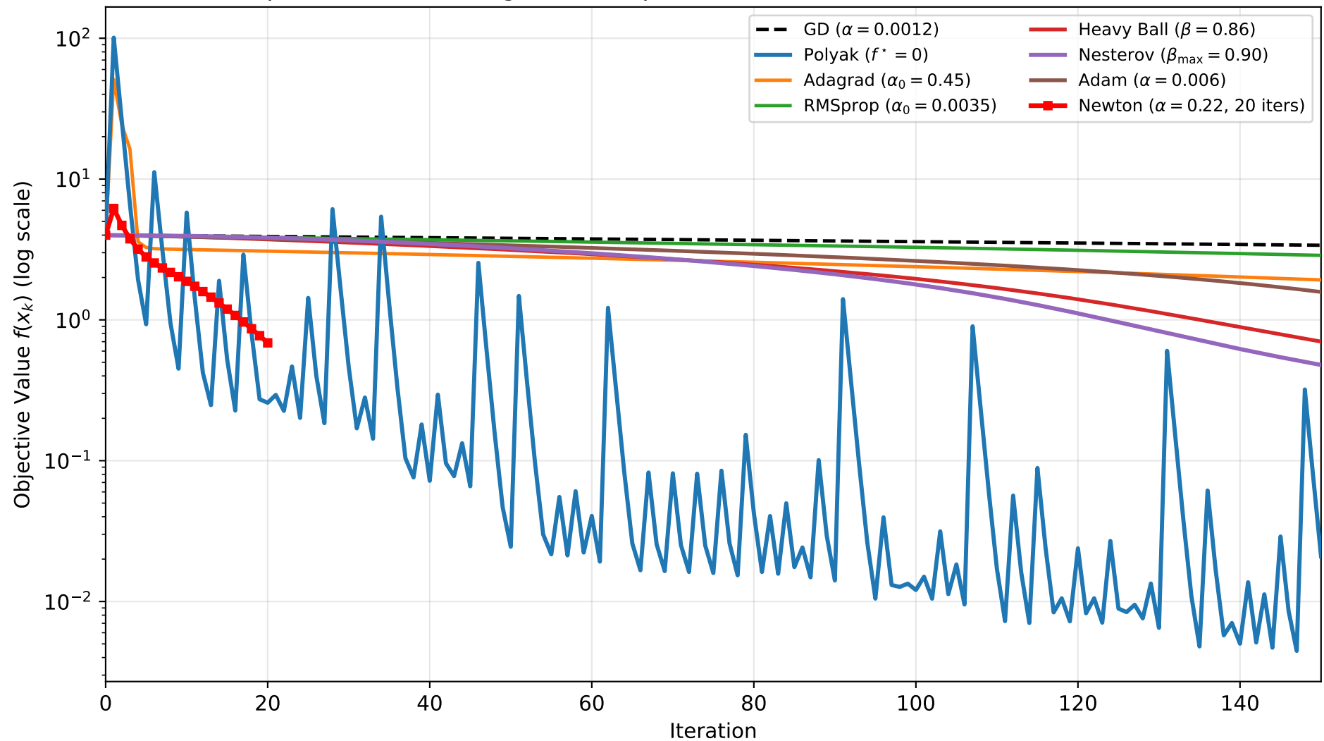
Comprehensive Convergence Comparison: Benchmark C (Rosenbrock, \kappa \approx 2504 )
