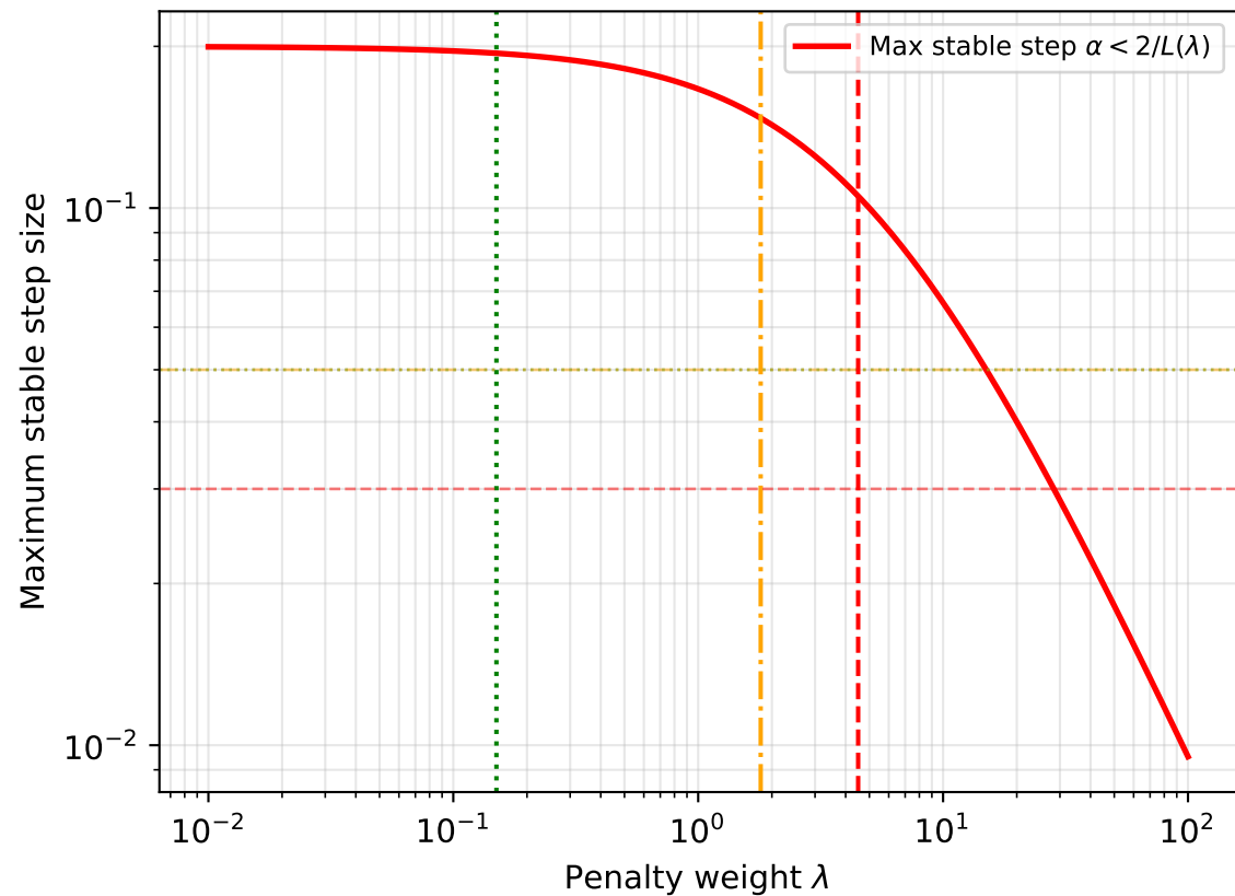
Q5: Maximum Stable Step Size vs Penalty Weight \lambda
