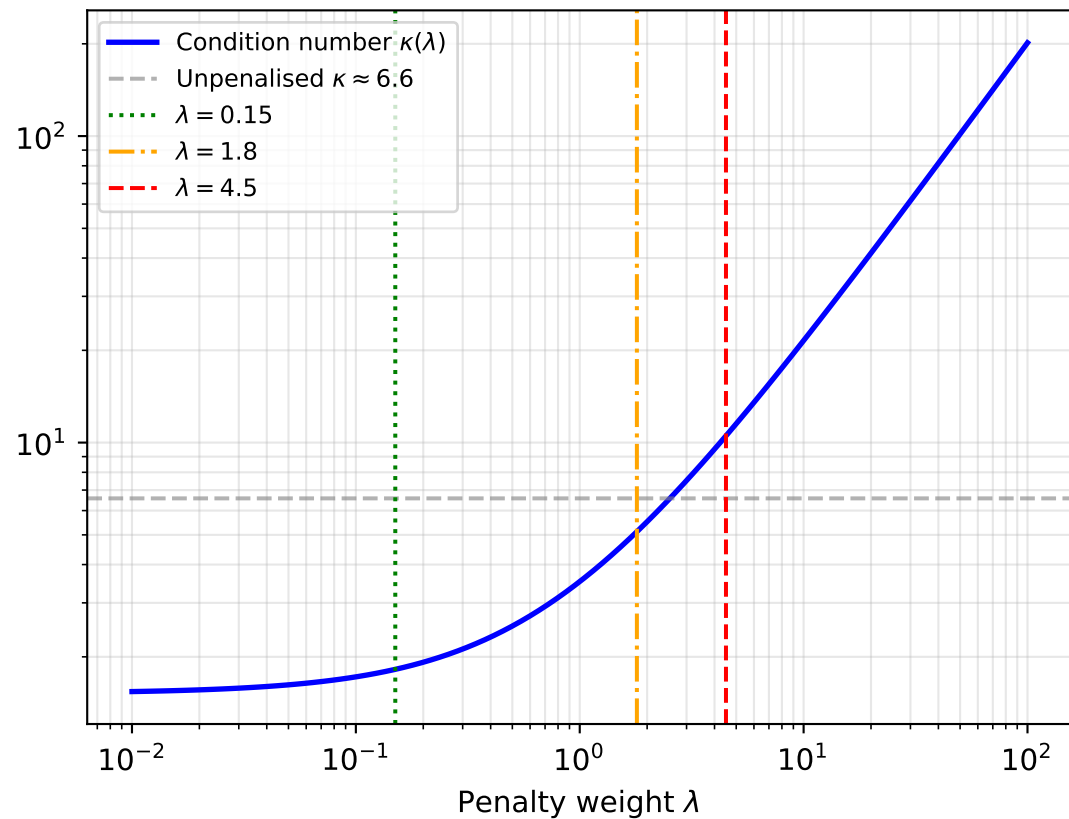
Q5: Penalty Method Condition Number Growth with \lambda
