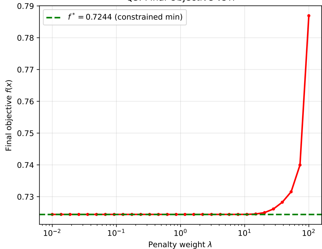
Q5: Final Objective vs \lambda
