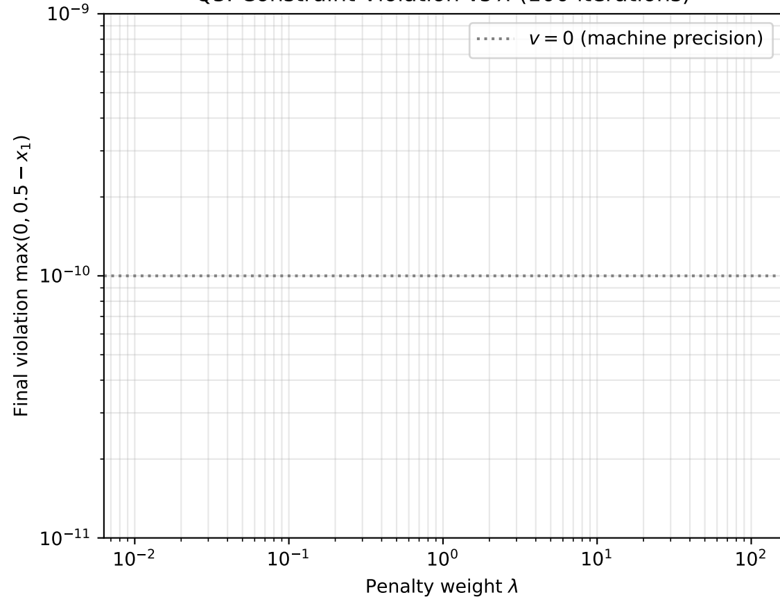
Q5: Constraint Violation vs \lambda (100 iterations)
