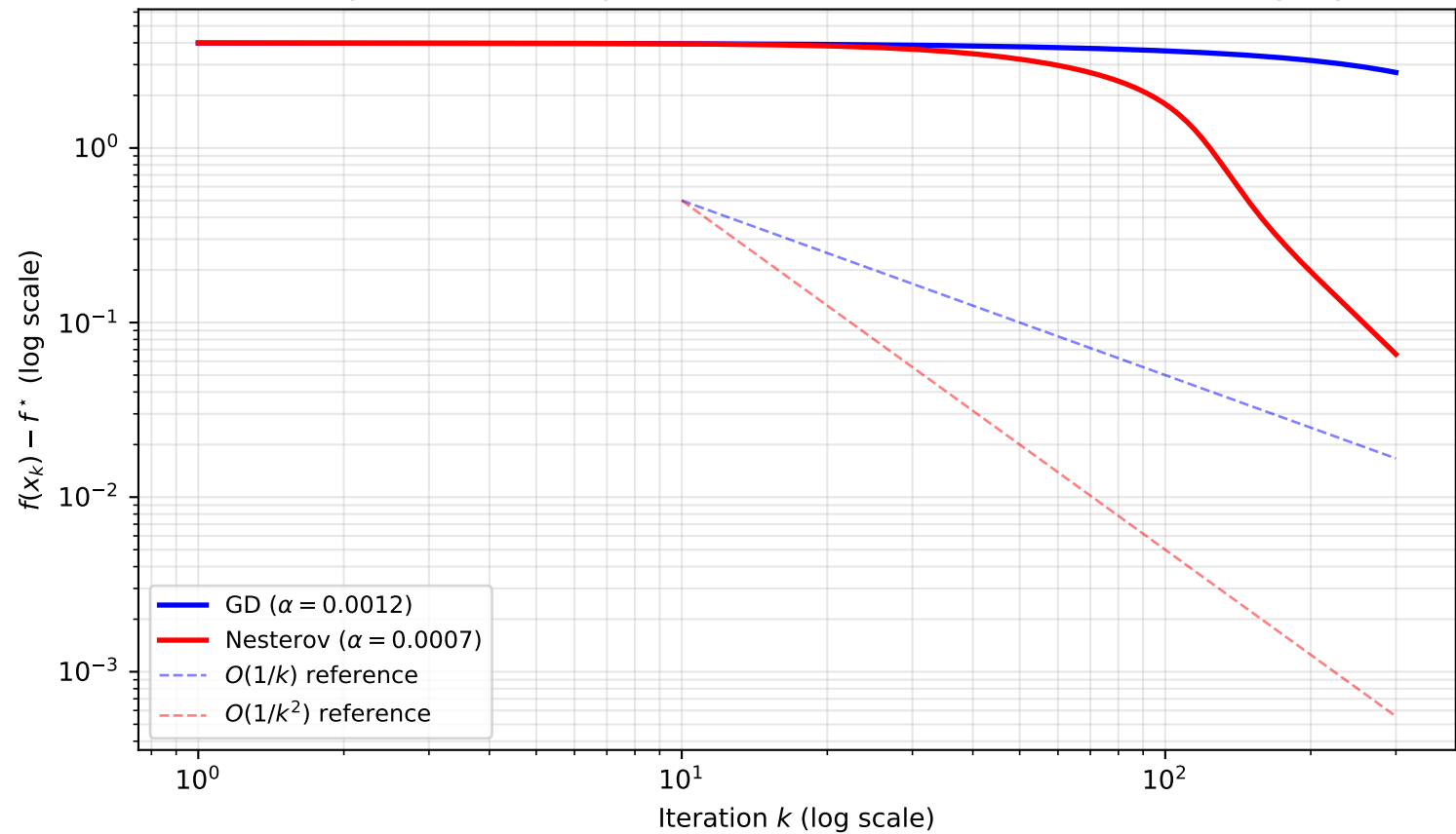
Convergence Rate Comparison: GD vs Nesterov on Rosenbrock (log-log)
