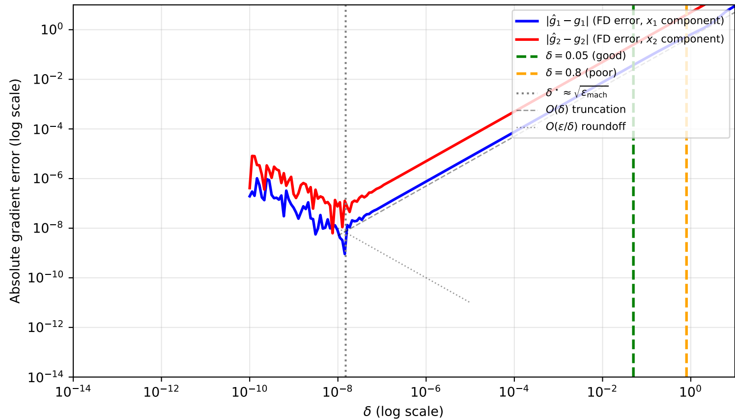
Q4: Finite Difference Error vs Step Size \delta (Benchmark B at x = (0.5, 2.5) )
