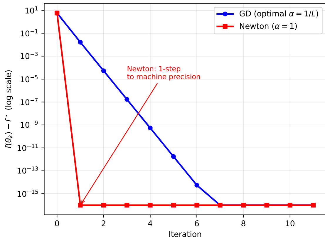
Quadratic Loss: Newton One-Step Convergence f^* reached after k = 1 (quadratic loss)
