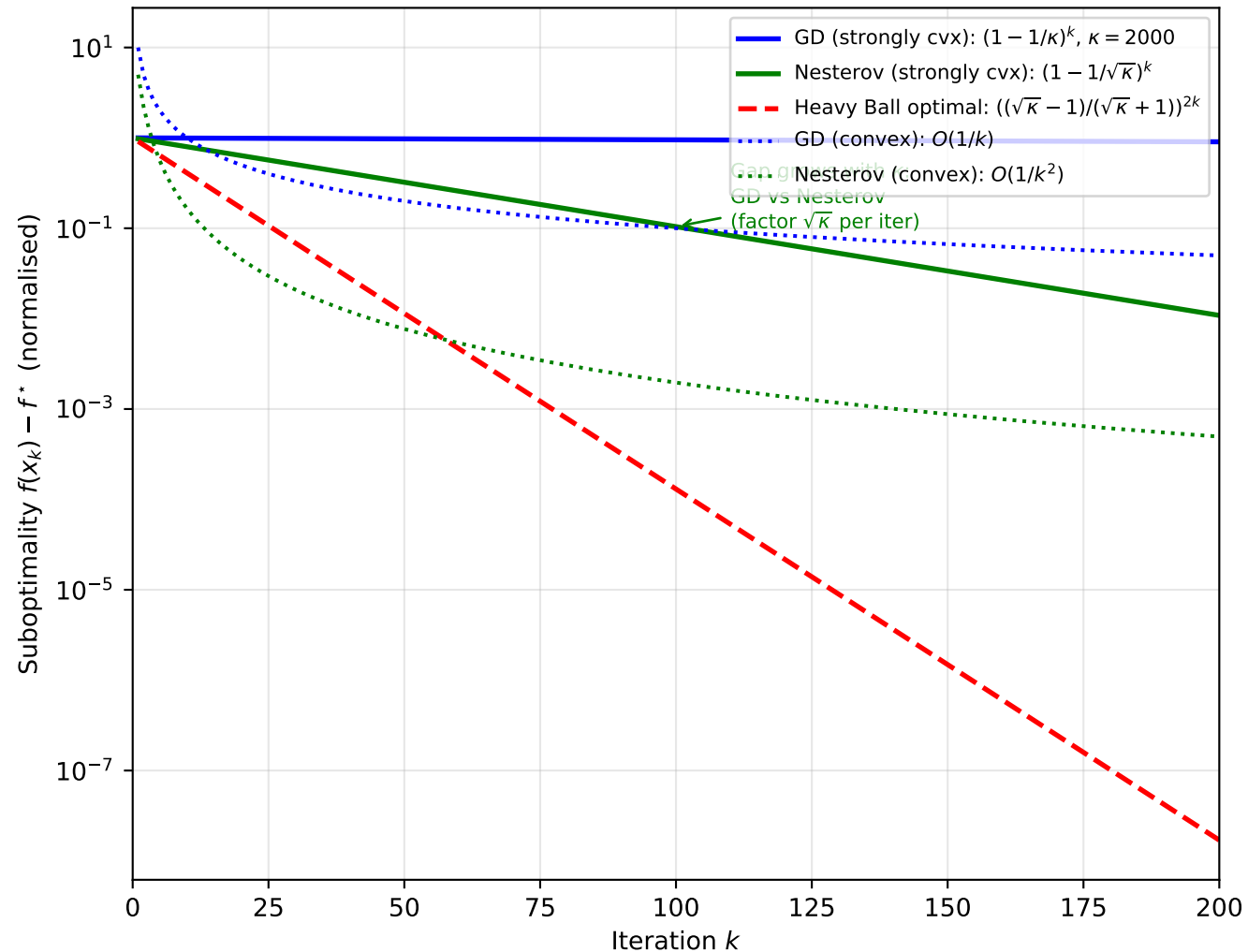
Theoretical Convergence Rates ( \kappa = 2000 , Rosenbrock regime)
