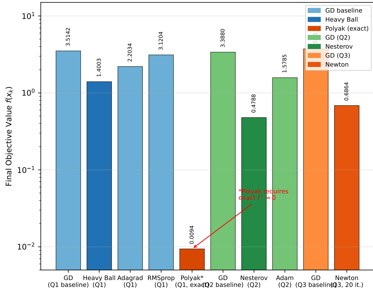
Benchmark C (Rosenbrock, \kappa \approx 2000 ): All Methods Final Values
