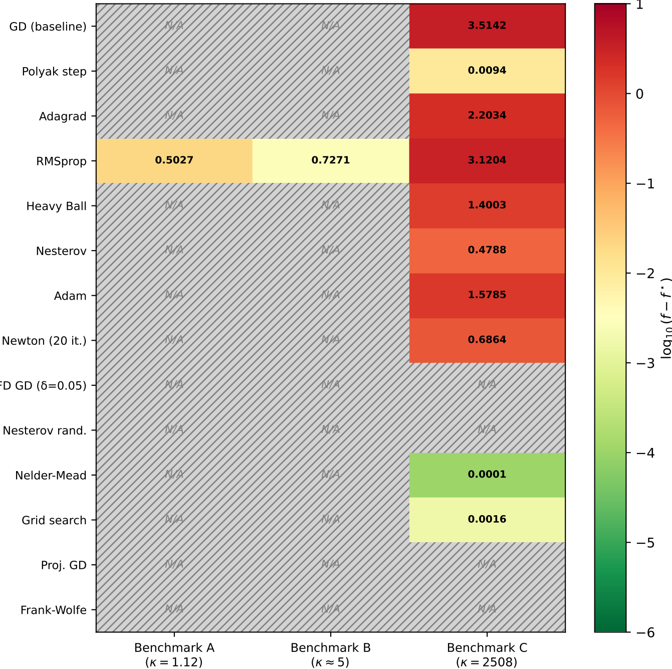
Method Performance Matrix (colour = \log_{10}(f - f^*) , green = better)
