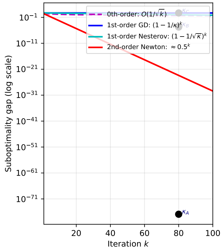
Oracle Information Hierarchy ( \kappa = 2508 , \|x_0 - x^*\| = 2 )
