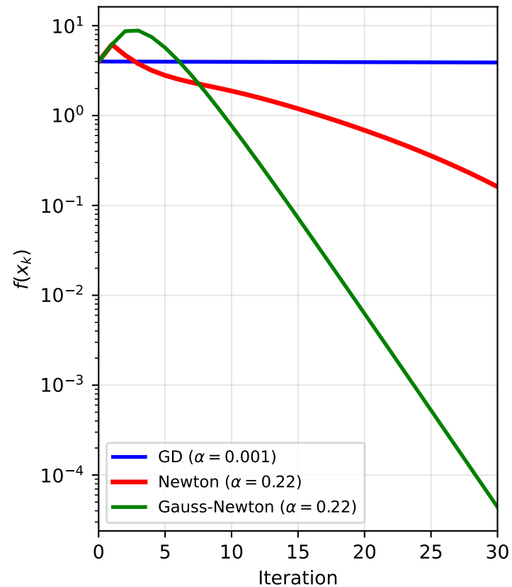
Gauss-Newton vs Newton vs GD (Benchmark C, Rosenbrock)
