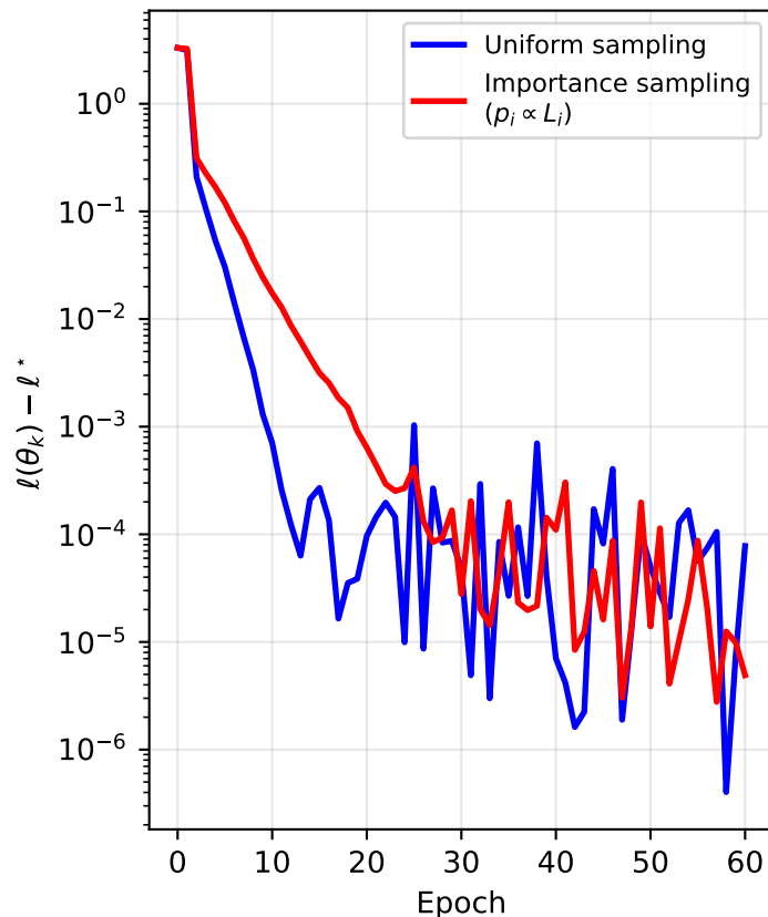
SGD Importance Sampling (reduces effective \kappa )
