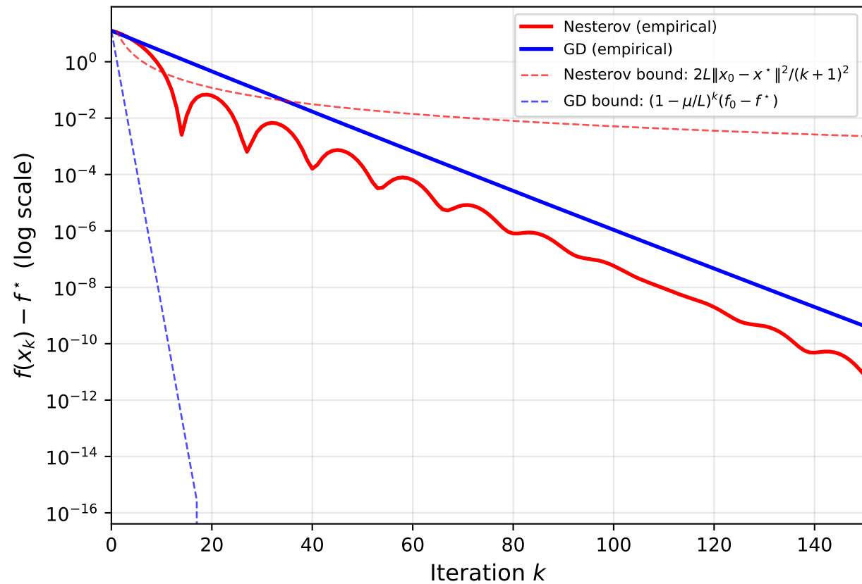
Nesterov vs GD: Empirical Convergence vs Theoretical Bounds on Benchmark A
