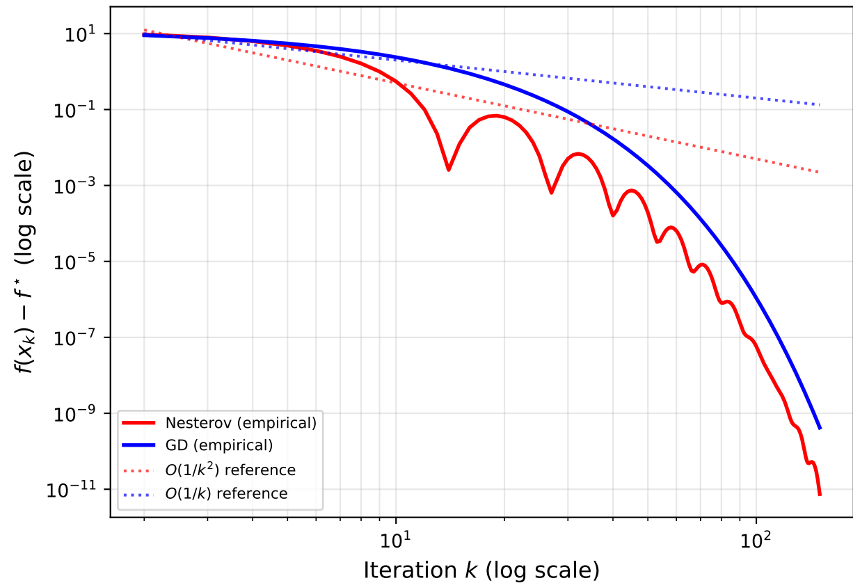
Log-Log Convergence Rate: O(1/k^2) vs O(1/k) on Benchmark A
