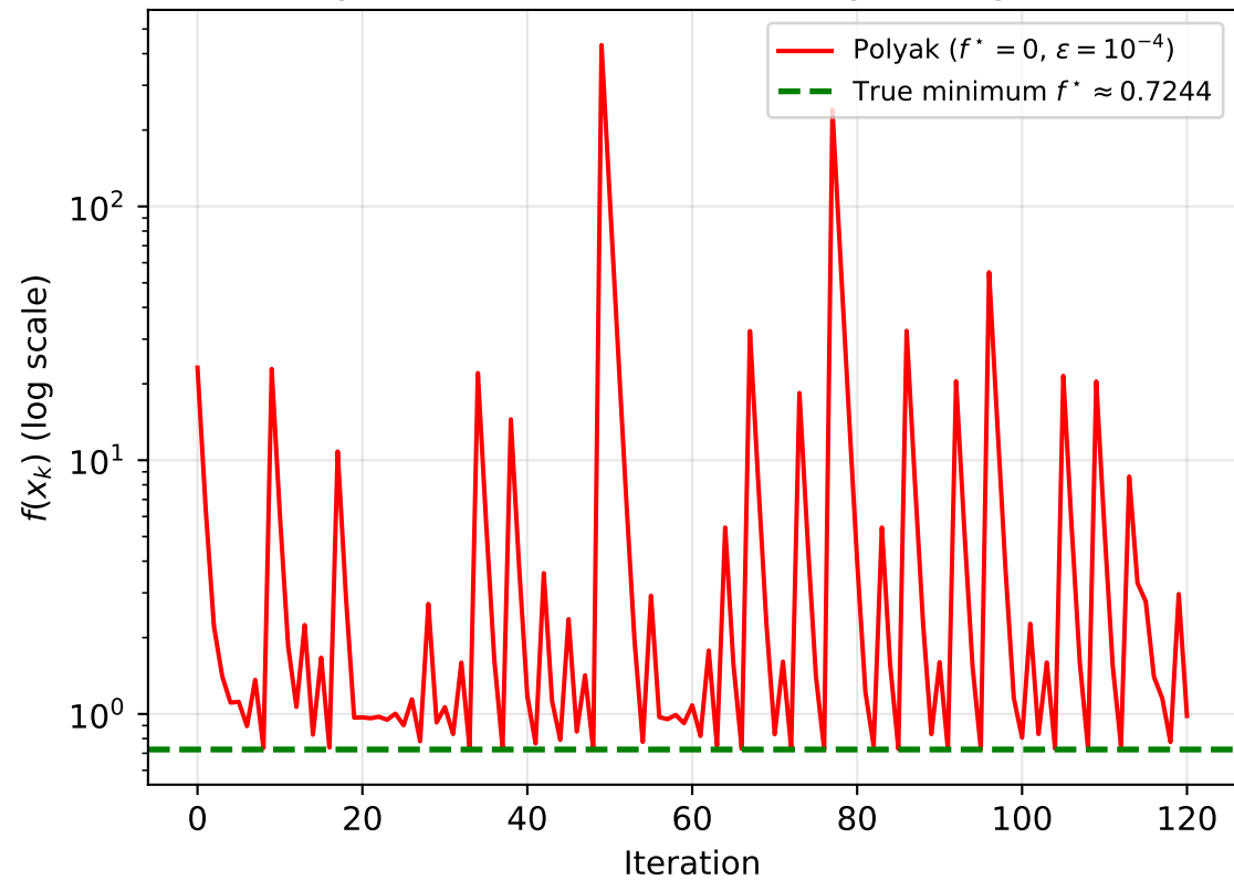
Polyak on Bench B: Oscillatory Divergence
