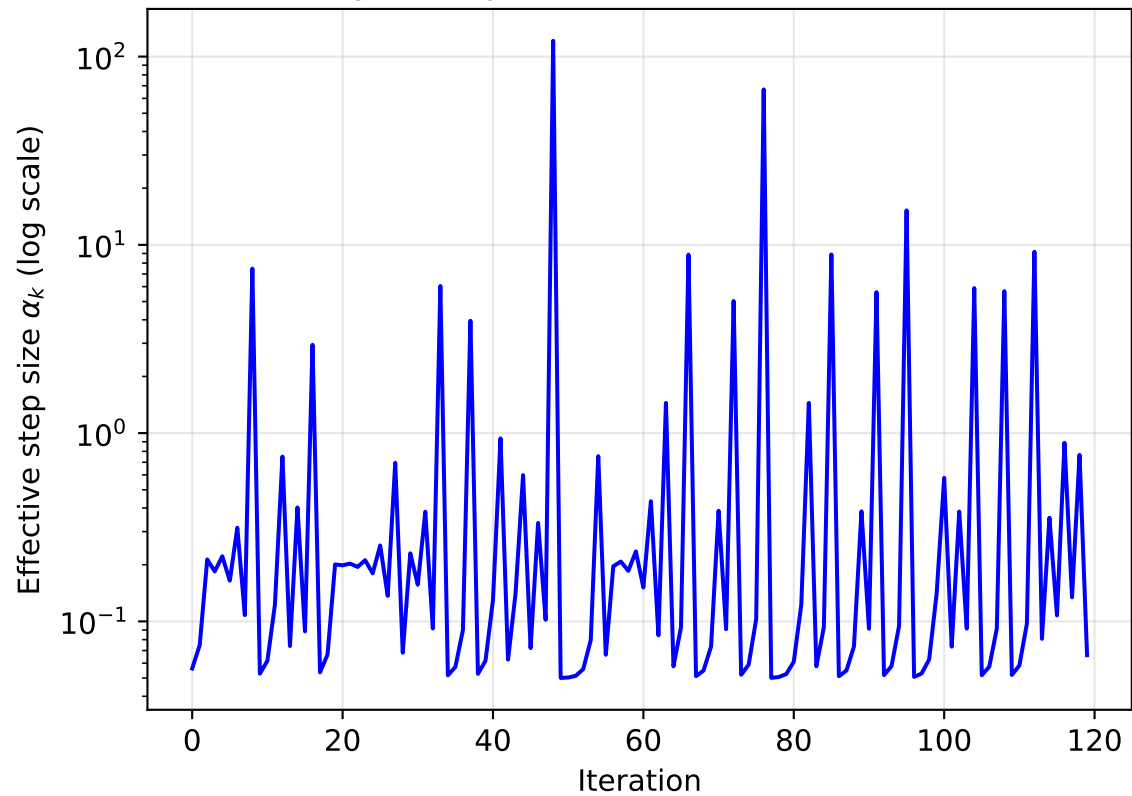
Polyak Step Size Evolution on Bench B
