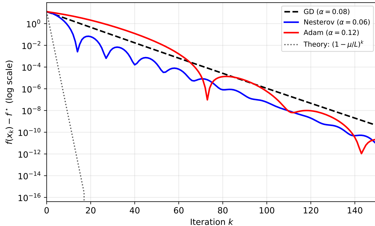
Convergence on Benchmark A: f(x_k) - f^* vs k
