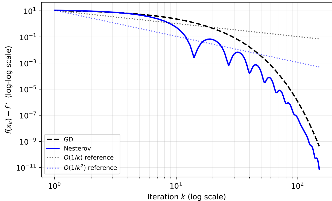
Log-Log: Convergence Rates on Benchmark A
