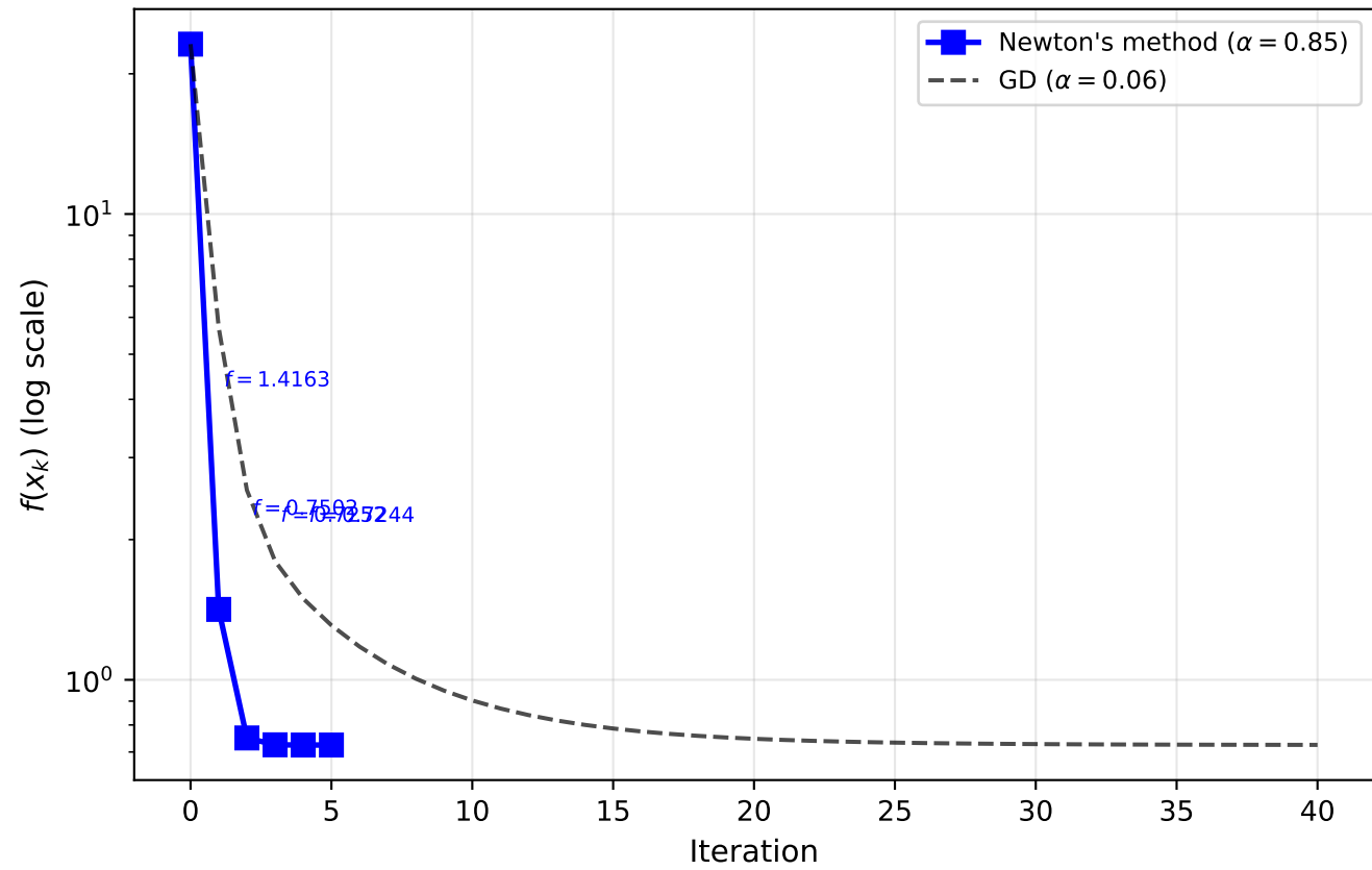
Newton vs GD on Benchmark B (Quadratic Convergence Visible)
