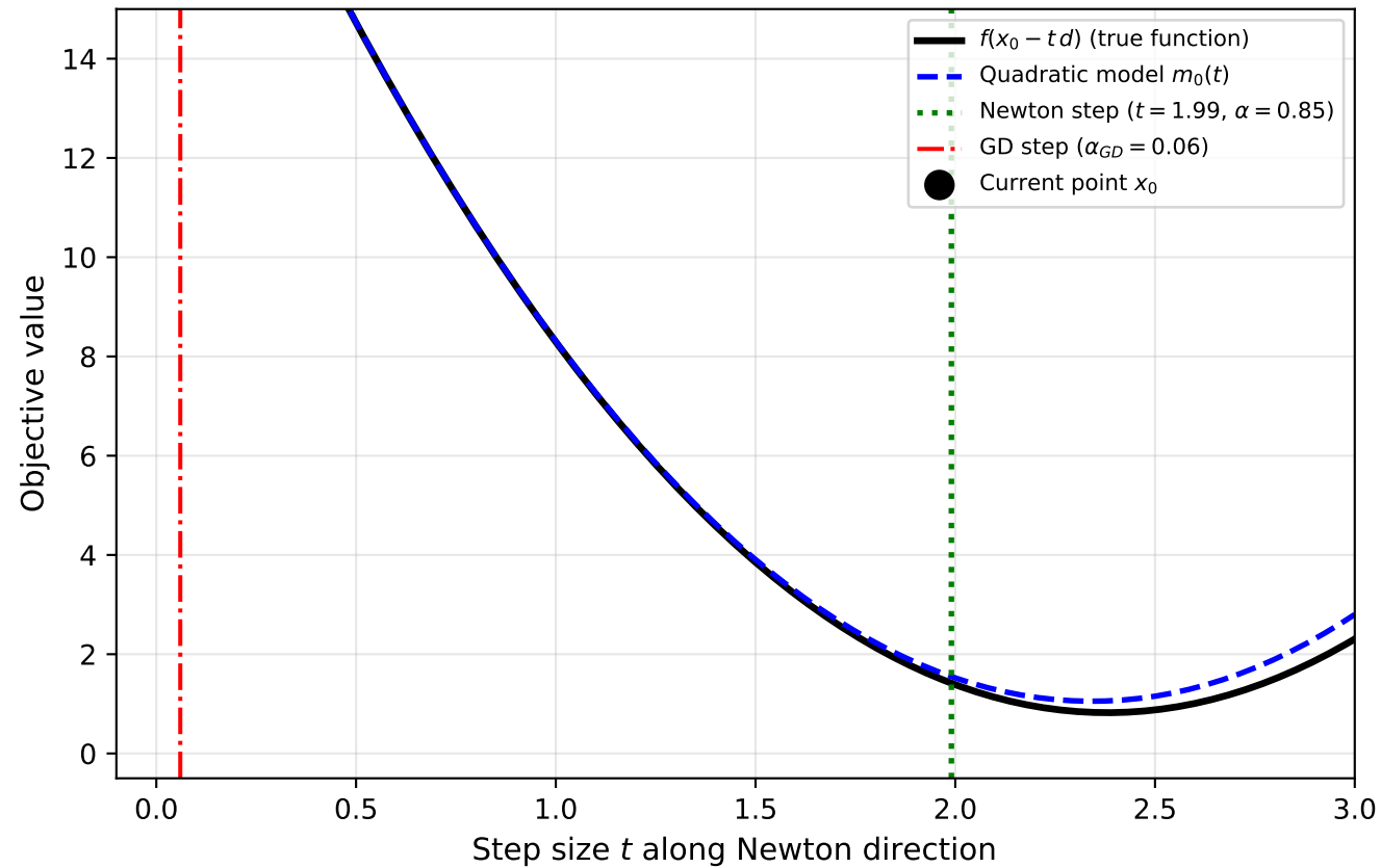
Newton's Method: Quadratic Model vs True Function (Benchmark B, step 0)
