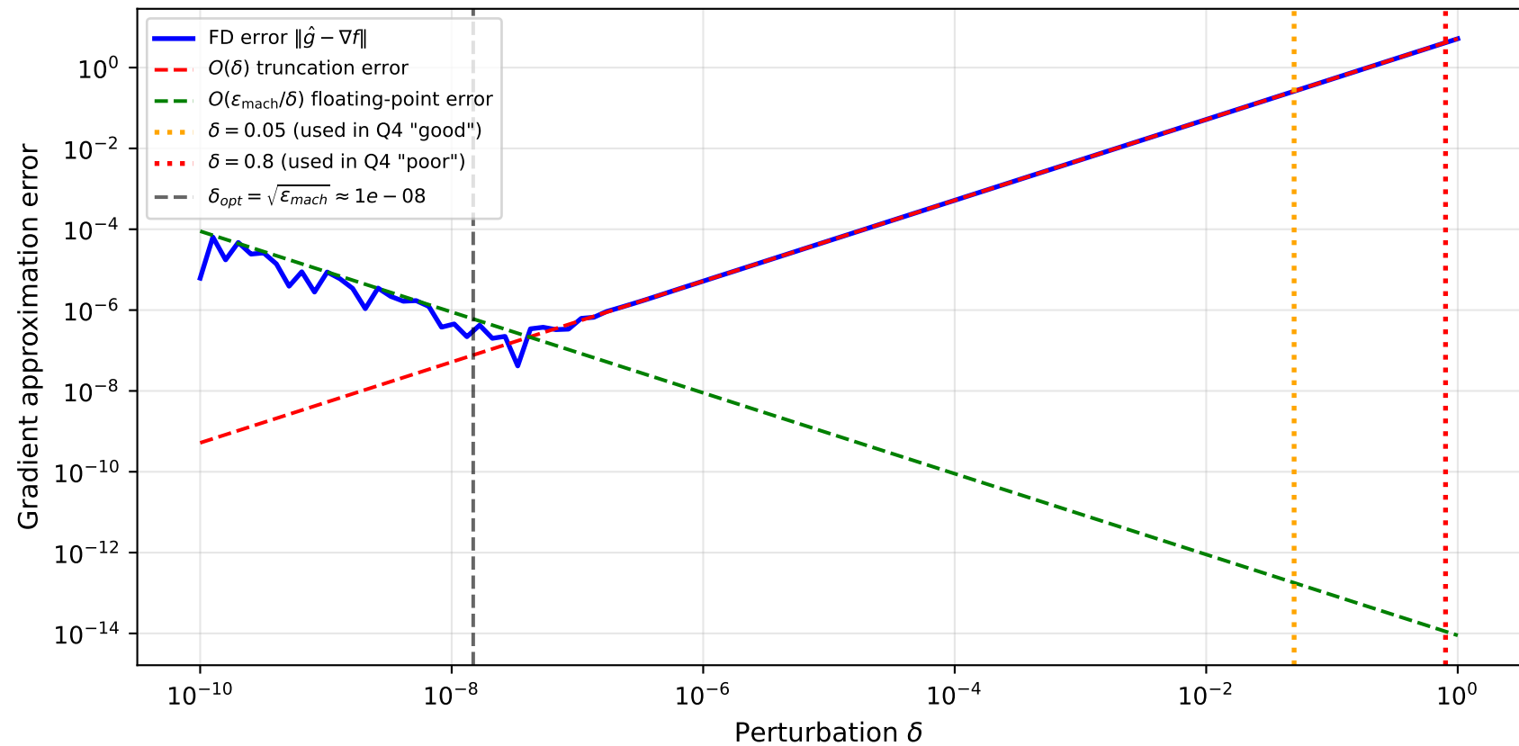
Q4: Finite Difference Error vs Perturbation Size (Benchmark B at x_0 = [-1, 4]^T )
