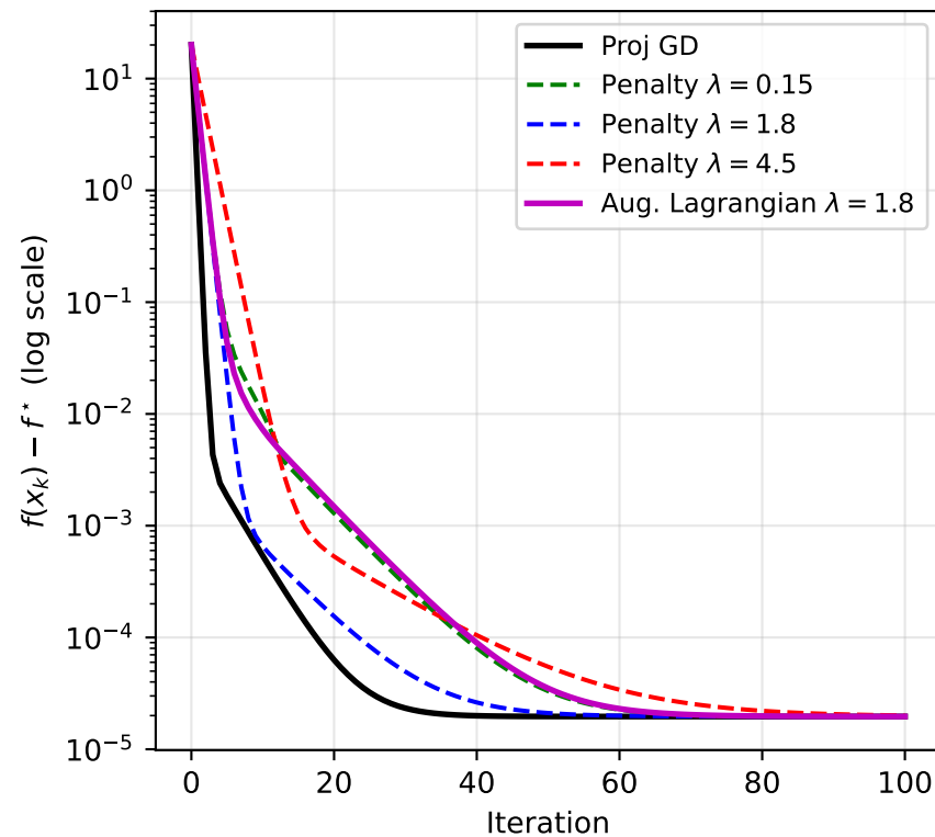
Q5: Objective Convergence (all methods)
