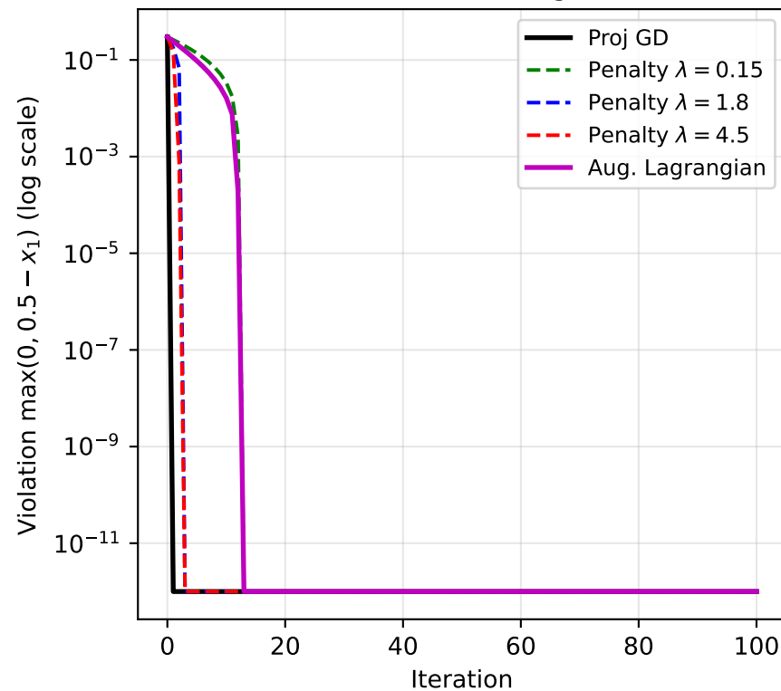
Q5: Constraint Violation All methods converge to 0
