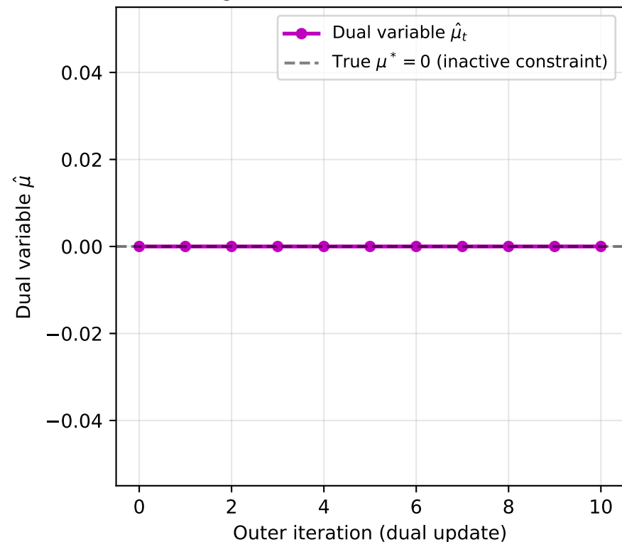
Aug. Lagrangian: Dual Variable (converges to 0 since constraint inactive)
