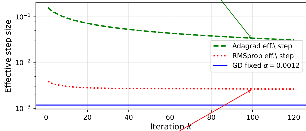
Effective Step Size: Adagrad vs. RMSprop (Benchmark C)
