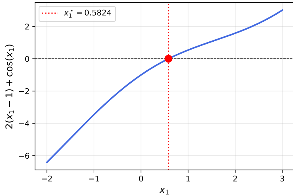
Optimality condition for Benchmark B \nabla_1 f = 0 \Leftrightarrow 2(x_1 - 1) + \cos(x_1) = 0
