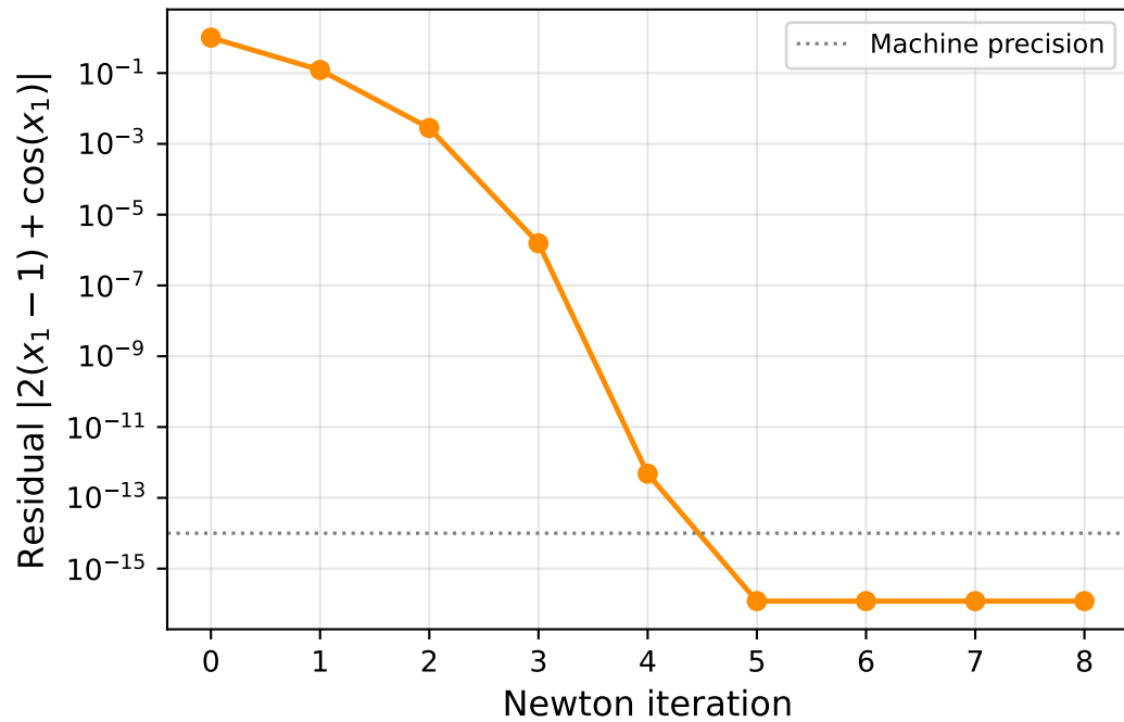
Newton root-finding for x_1^* converges quadratically to x_1^* \approx 0.5820
