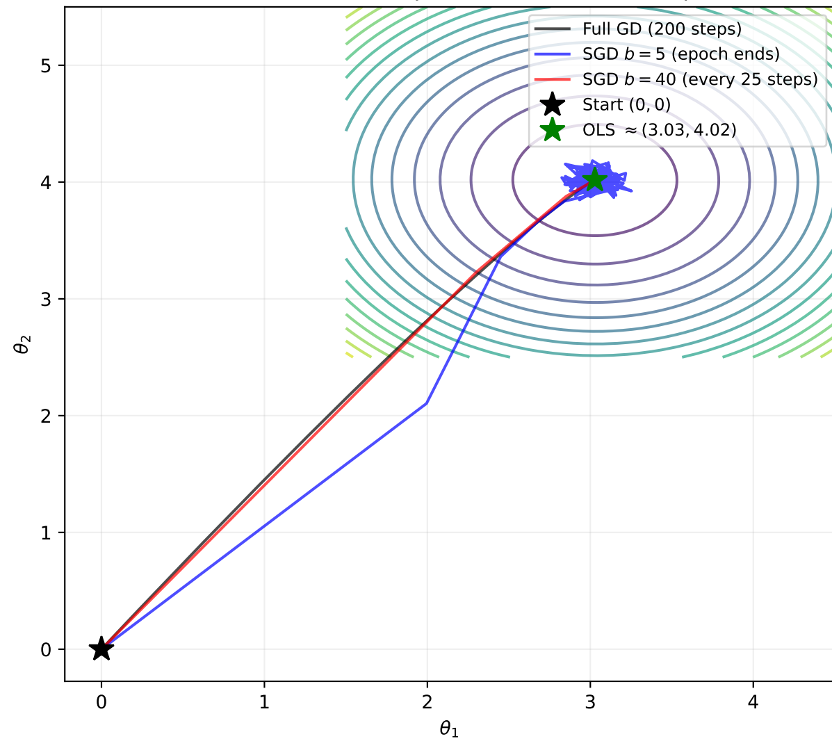
Q2: SGD vs Full GD Trajectories in Parameter Space
