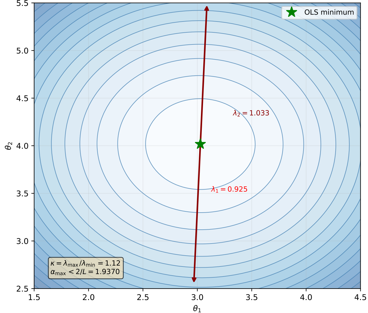
Bench A Hessian: \kappa = 1.12 , Principal Axes
