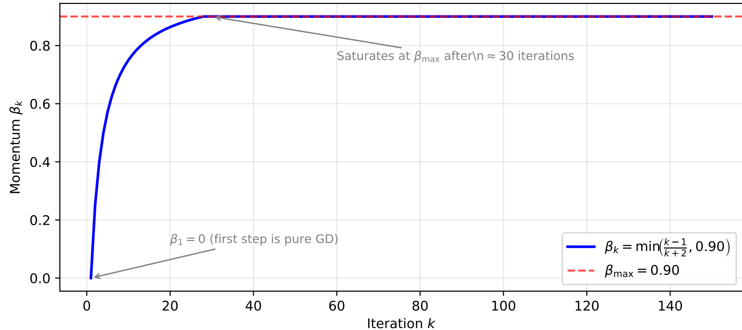
Q2: Nesterov Momentum Schedule \beta_k vs Iteration
