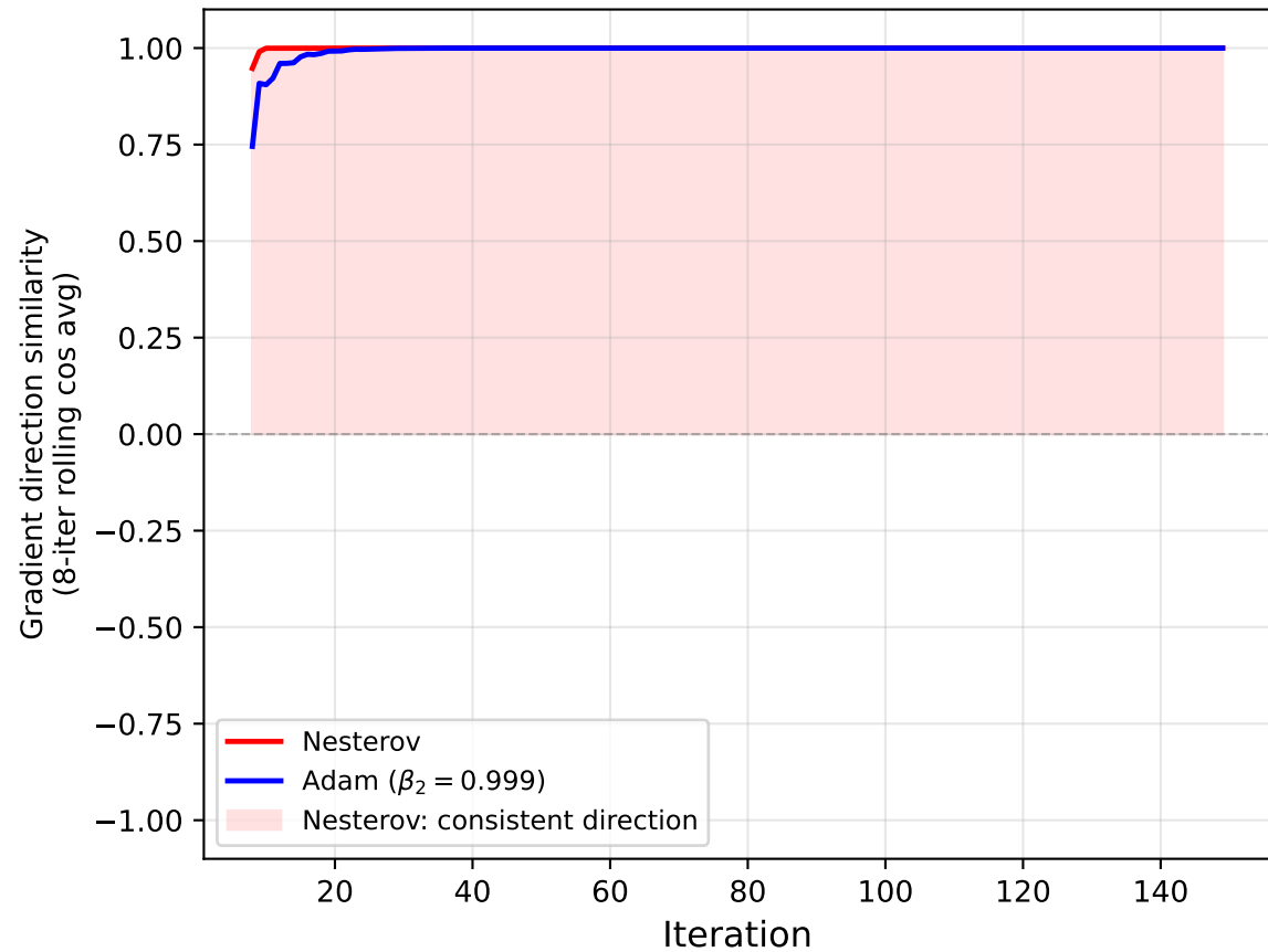
Gradient Direction Consistency
