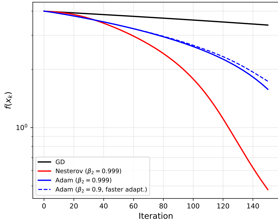
Q2: Convergence on Rosenbrock
