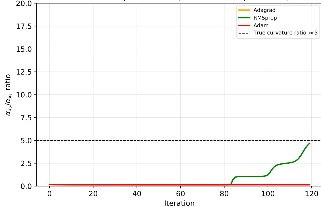
Effective Step Size Ratio (curvature compensation)
