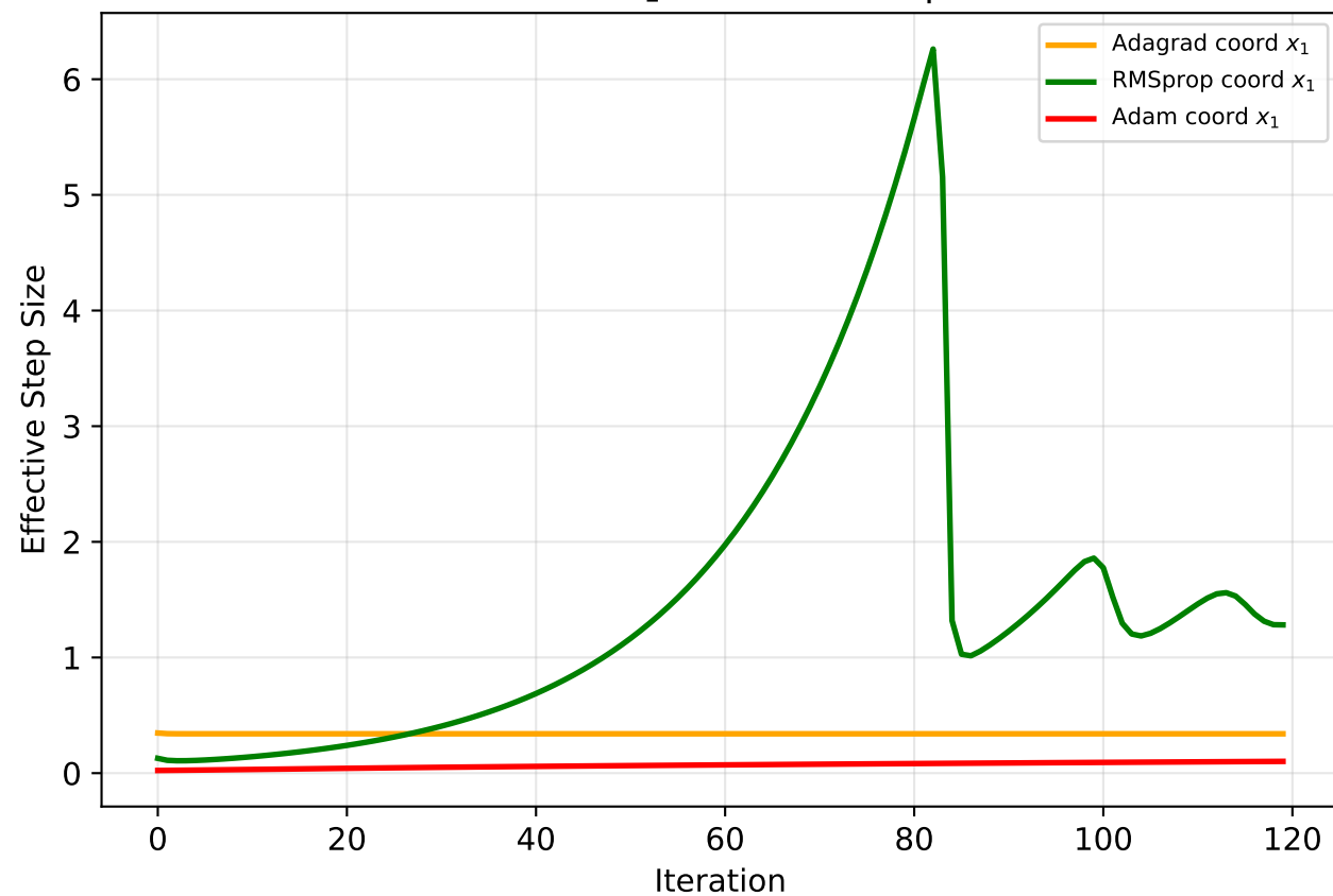
Effective Step Size Ratio (curvature compensation)
