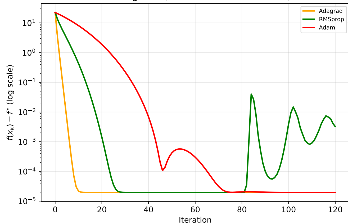
Convergence (Benchmark B, f^* = 0.7244 )
