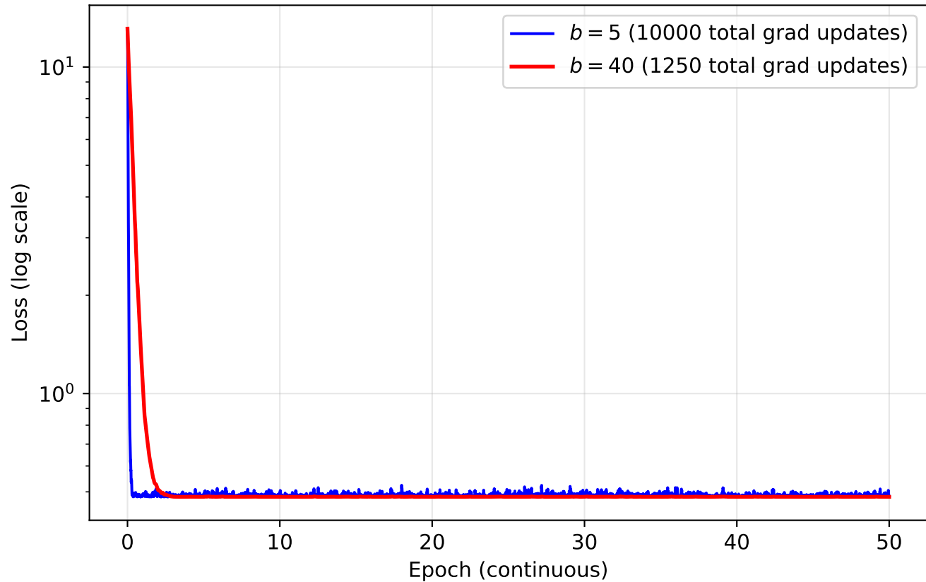
SGD: Loss per Gradient Update (same x-axis = epochs)
