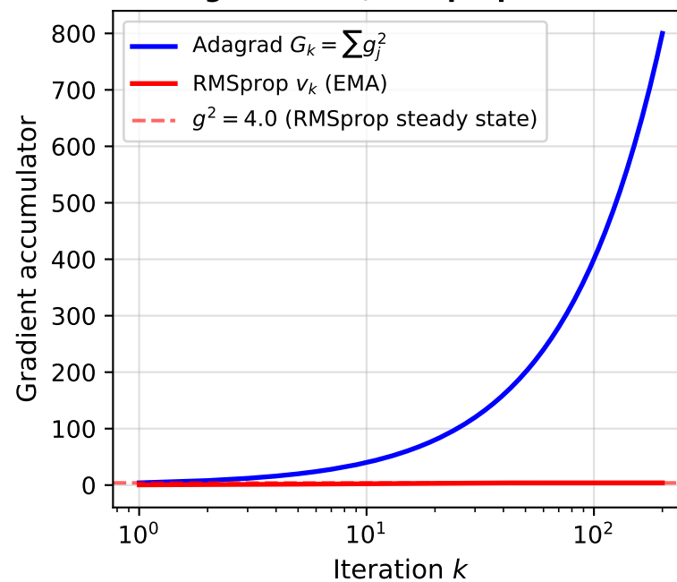
(b) Gradient accumulator growth (Adagrad linear, RMSprop bounded)
