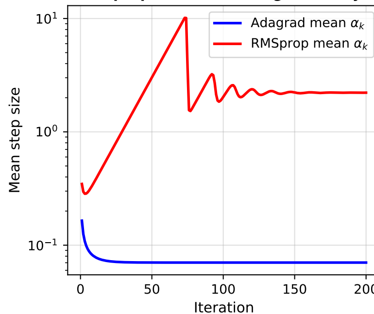
(e) Step size evolution on Benchmark A (RMSprop stabilises, Adagrad decays)
