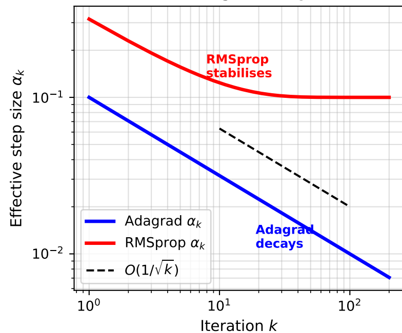
(a) Theoretical step decay (constant gradient g = 2 )
