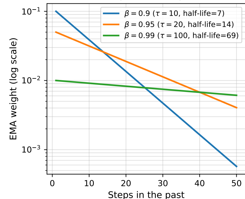
(f) RMSprop memory window ( k = 50 , weight of past gradients)
