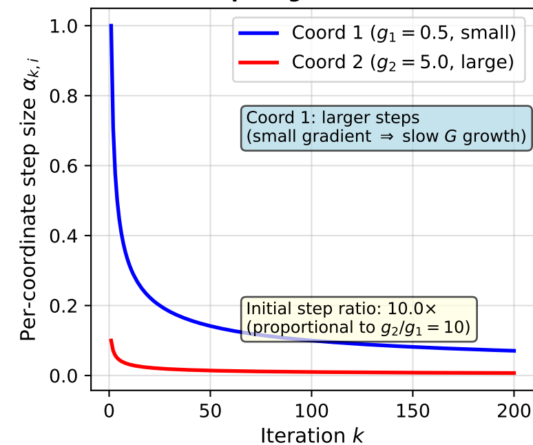
(c) Adagrad coordinate-wise adaptation (decoupled gradient scales)
