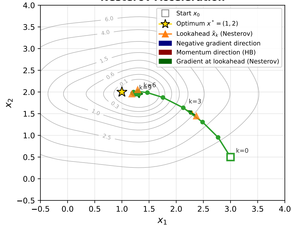
Nesterov Acceleration
