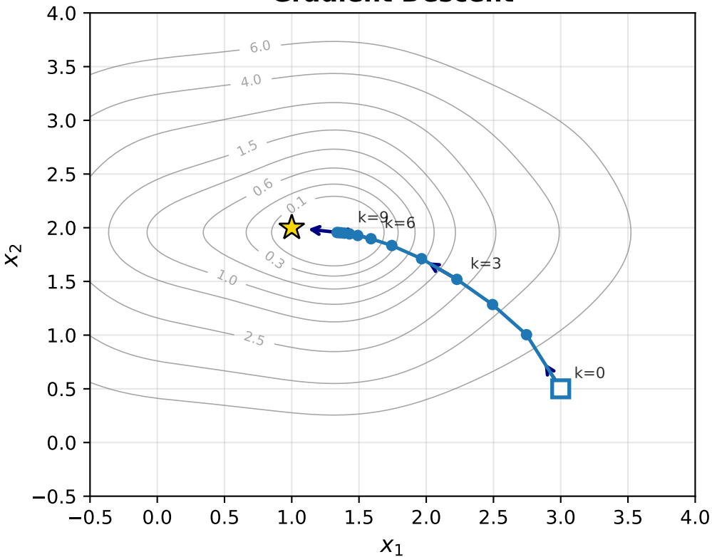
Gradient Descent
