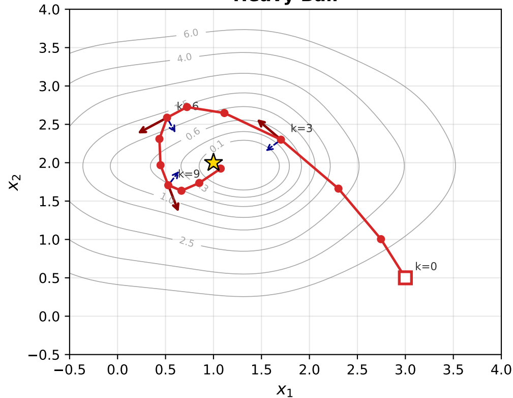
Heavy Ball
