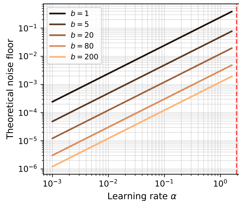
(c) Noise floor \propto \alpha/b (theoretical, \kappa = 1.1 )
