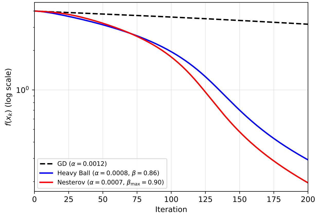
Q1/Q2: Heavy Ball vs Nesterov — Benchmark C (Rosenbrock, 200 iterations)
